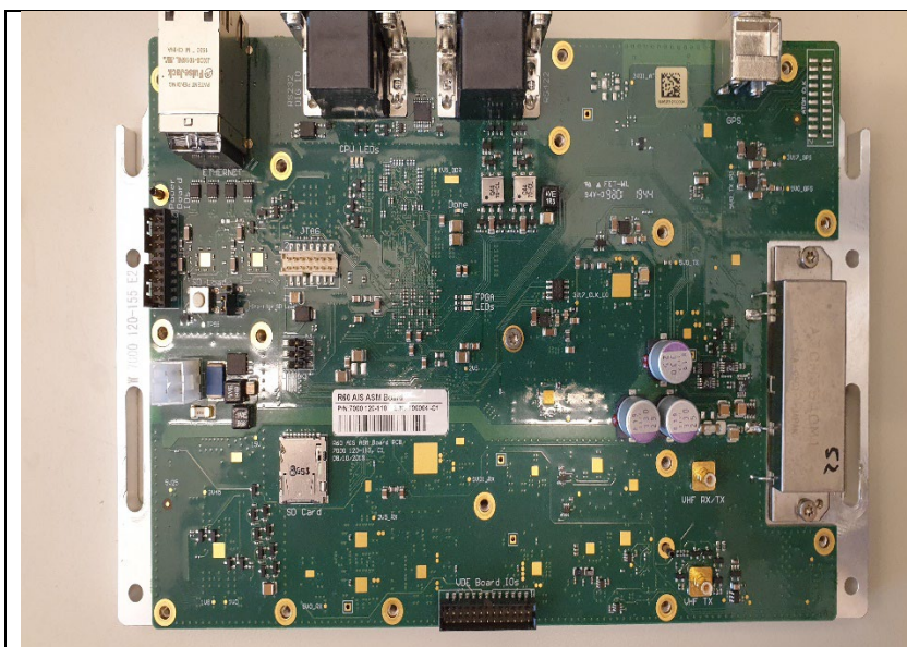
Figure 11: AIS PWB TOP Side View
