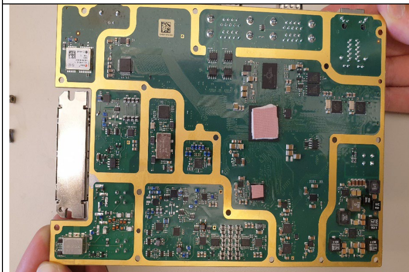
Figure 12: AIS PWB Bottom Side View
