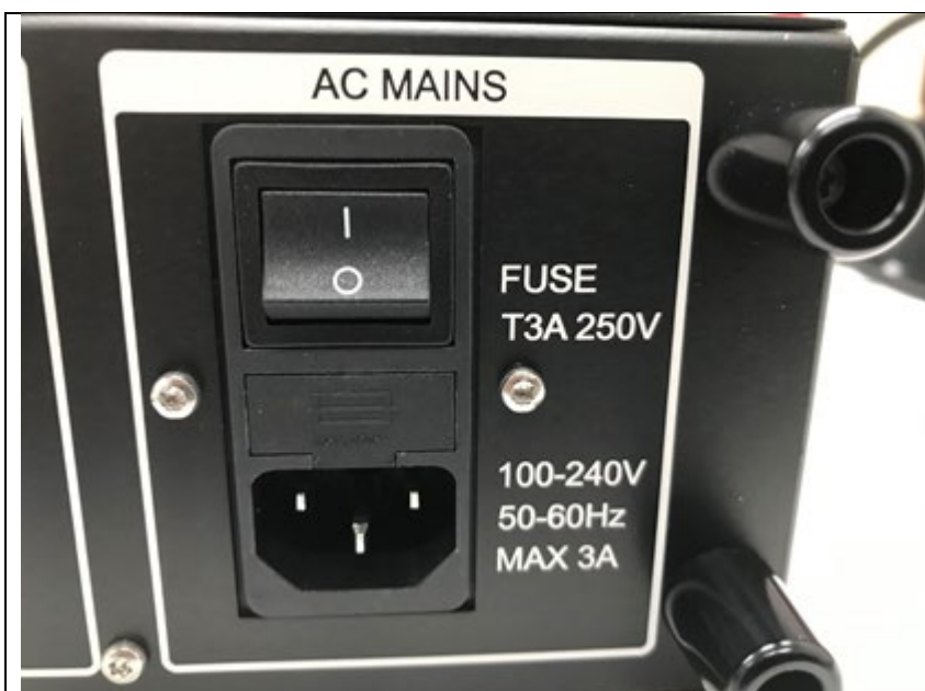
Figure 5: AC Main Connection and Main Fuse View
