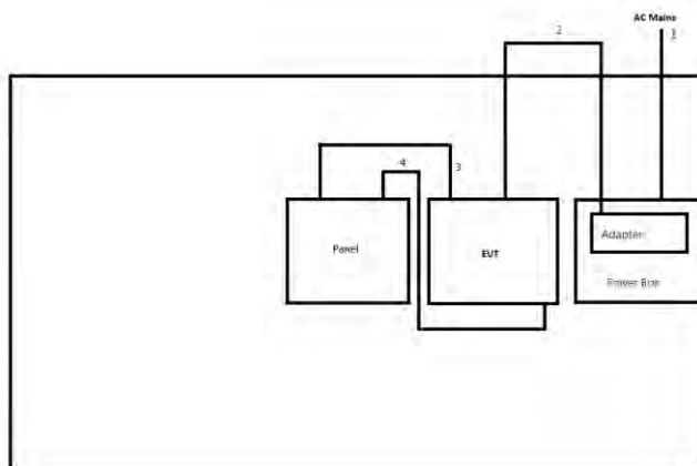
Test Setup Diagram - Radiated Test (Non-Beamforming_Panel)
