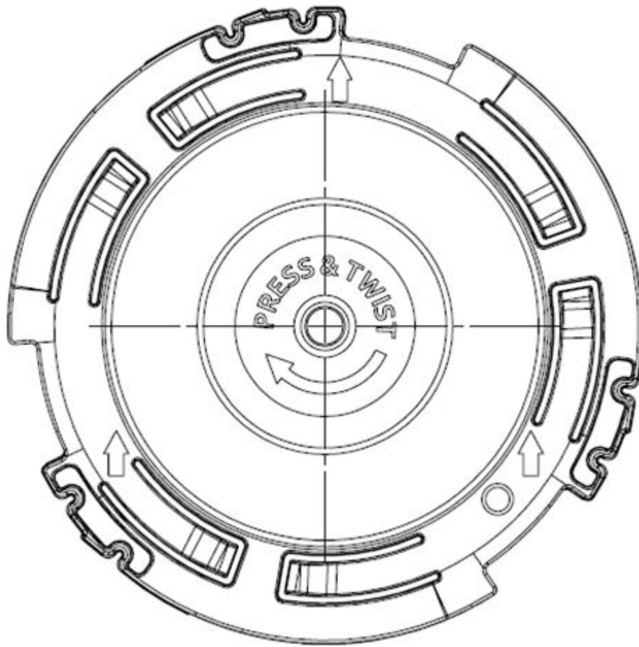
Figure 17: ACC-BKT-AX-JB Accessory Bracket Plastic Part
