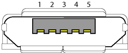
Figure 9: Micro-B model Console Port Pin Information
