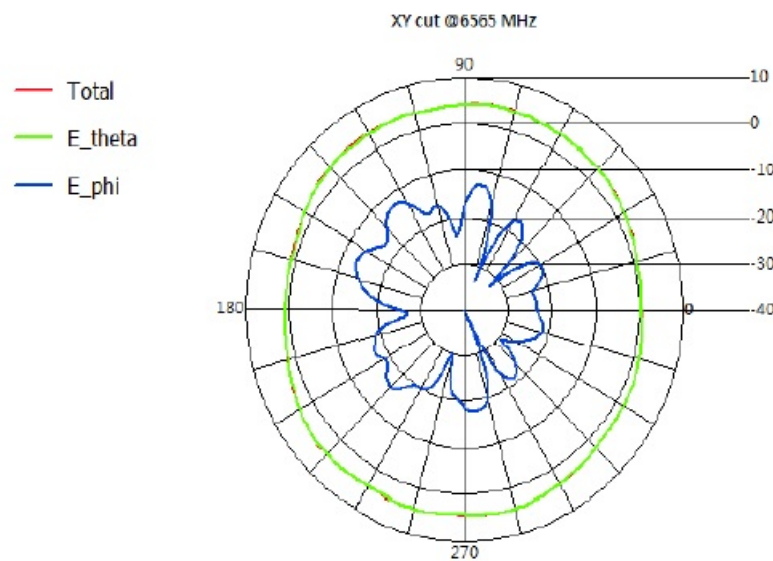
Figure 4: AP3000X Integrated Antenna 6.5GHz Radiation Pattern - Horizontal
