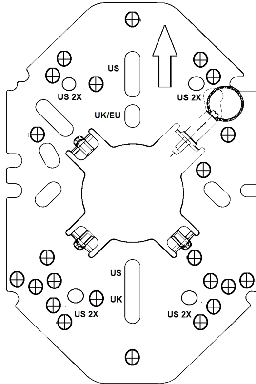
Figure 16: ACC-BKT-AX-JB Accessory Bracket Metal Part
