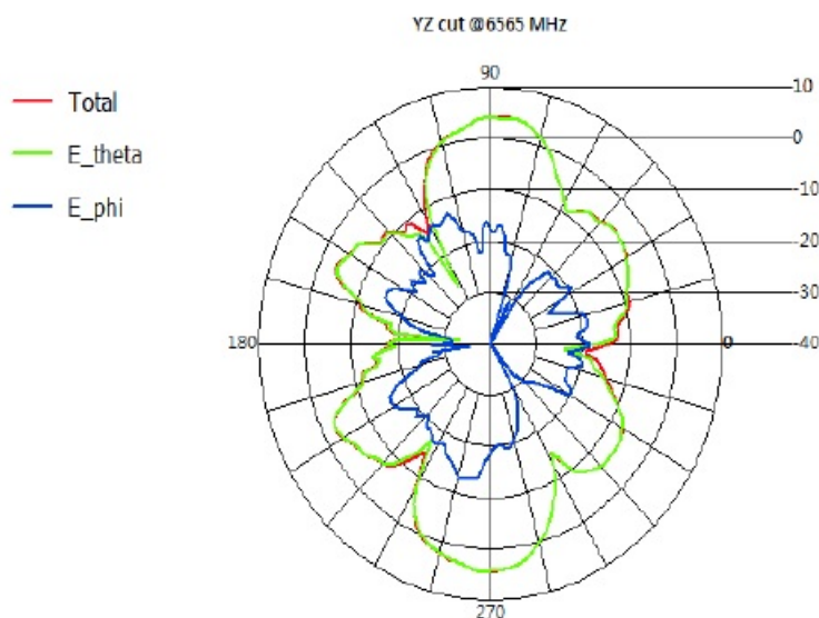
Figure 5: AP3000X Integrated Antenna 6.5GHz Radiation Pattern - Elevation
