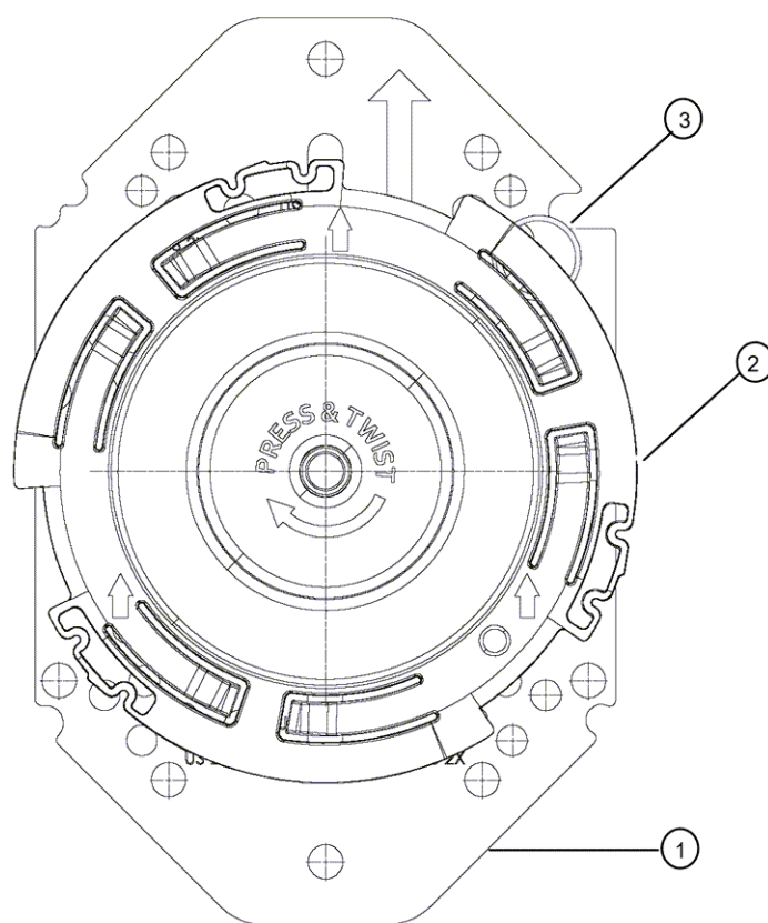
Figure 18: Junction Box Accessory Bracket Assembly
