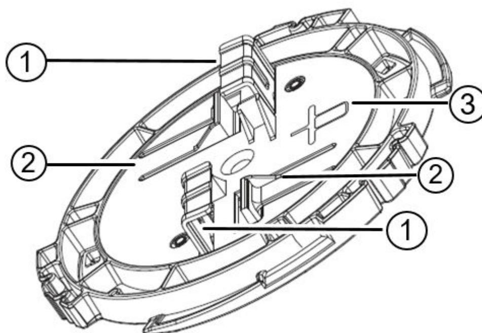
Figure 11: AH-ACC-BKT-AX-SL Accessory Bracket
