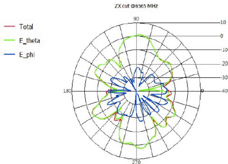
Figure 5: AP3000X Integrated Antenna 6.5GHz Radiation Pattern - Elevation
