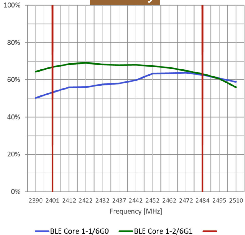
Efficiency
