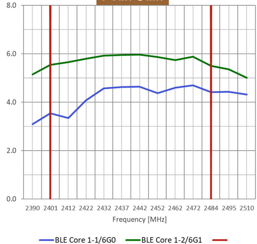
Peak Gain
