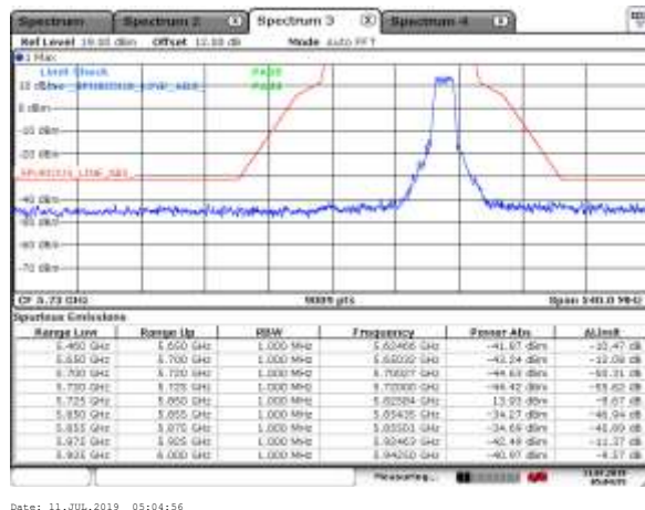
5825MHz with SISO
