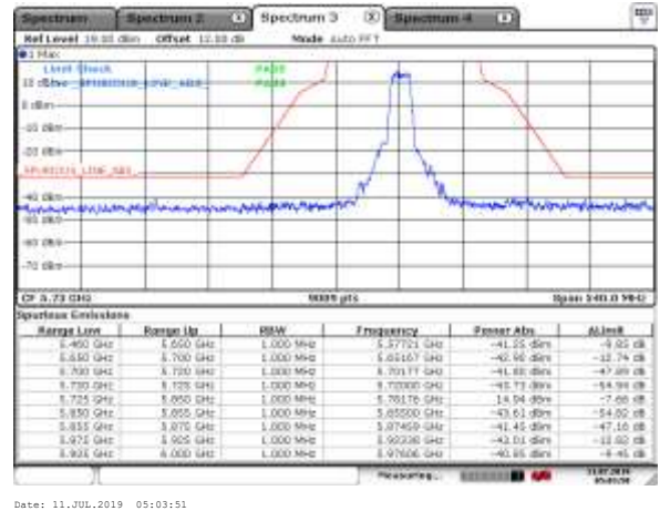
5785MHz with SISO
