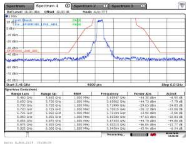
5745MHz with CDD
