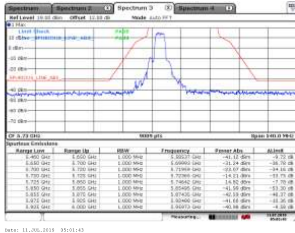
5745MHz with SISO
