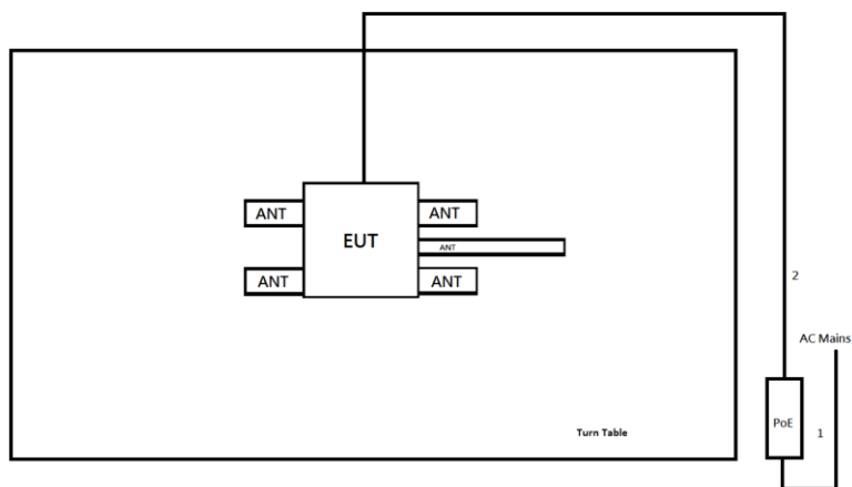
Test Setup Diagram - Radiated Test (Sample 2) Dipole
