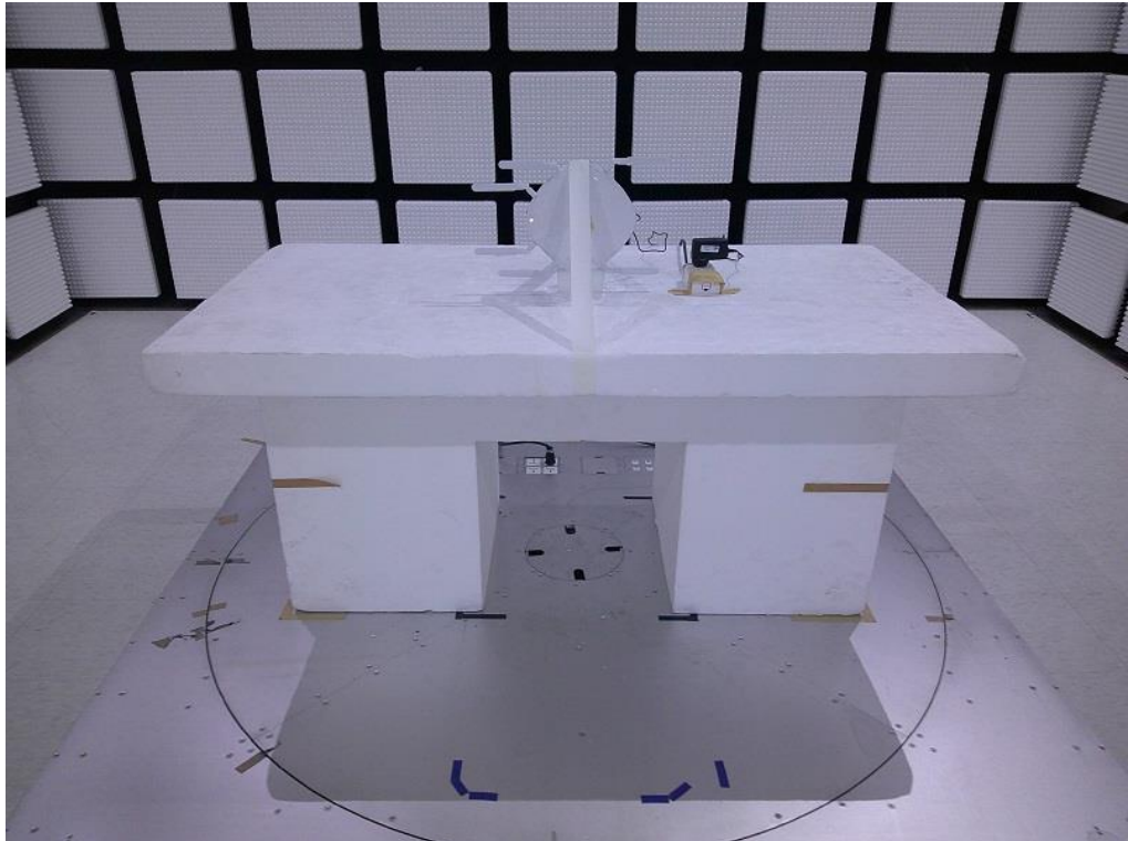
Radio 1 Dipole Antenna (2T1S)
