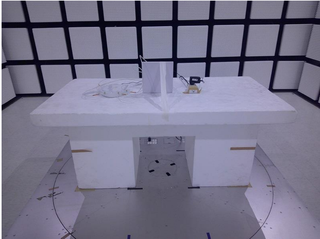
Radio 1 Dual-Polarized MIMO Panel Antenna (1T1S)
