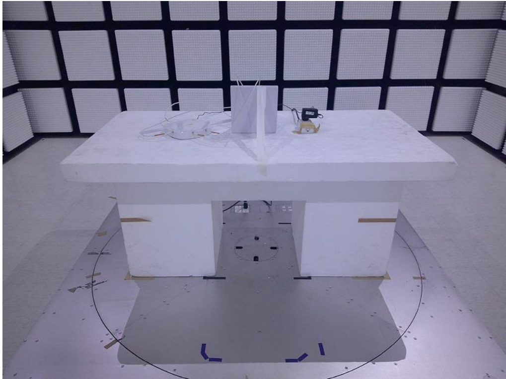
Radio 1 Dual-Polarized MIMO Panel Antenna (2T2S)
