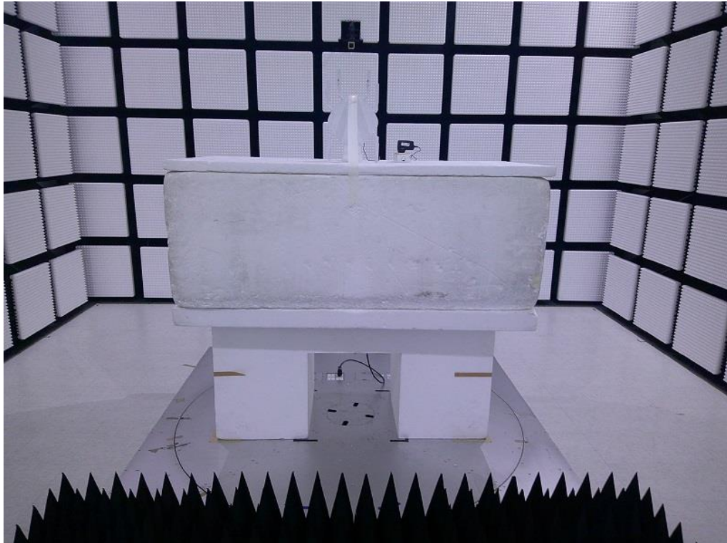
Radio 1 Dipole Antenna (2T2S)
