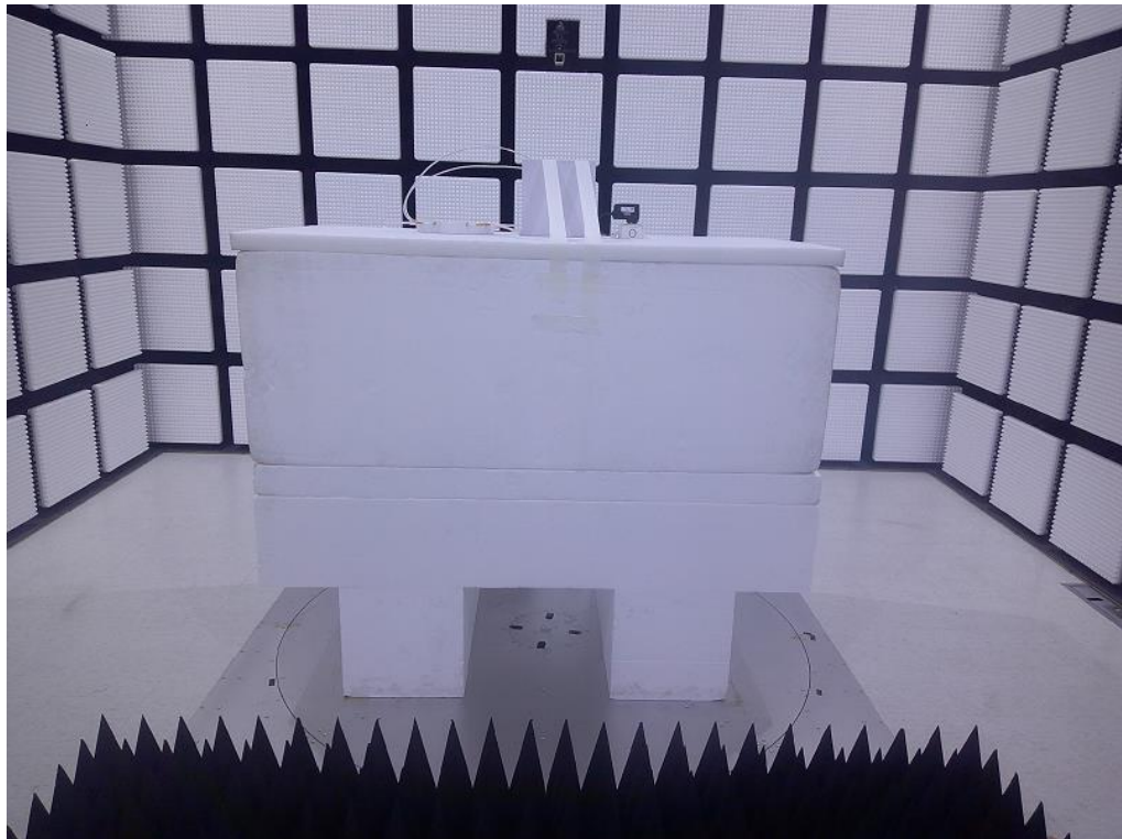
03CH02-HY Radio 3 Dual-Polarized MIMO Panel Antenna (2T2S)
