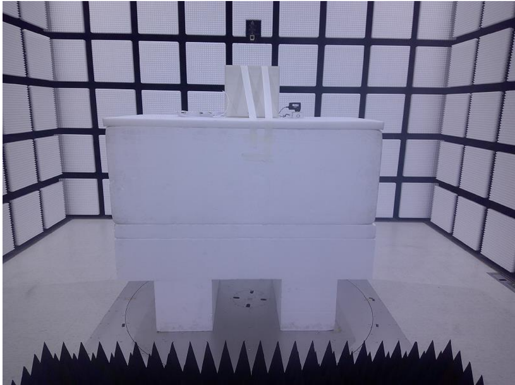
Radio 3 Dual-Polarized MIMO Panel Antenna (1T1S)
