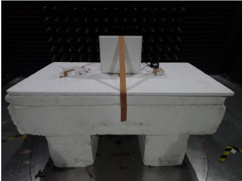
Radio 3 MIMO-directional Antenna (1T1S)
