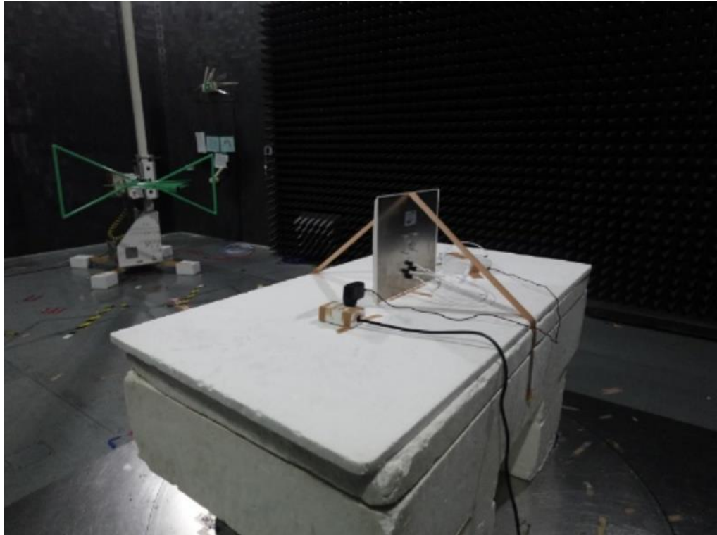
Radio 2 MIMO-directional Antenna (1T1S) and (2T1S)
