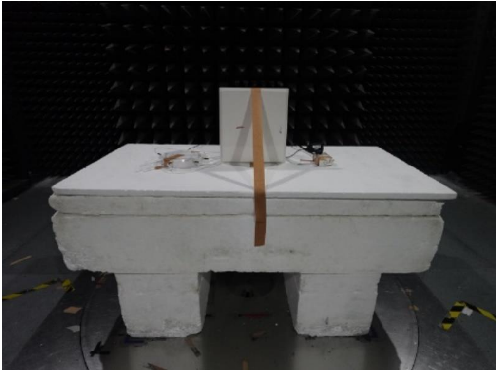
Radio 2 MIMO-directional Antenna (2T2S)
