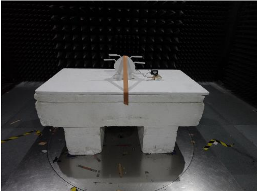
Radio 2 Dipole Antenna (2T1S)
