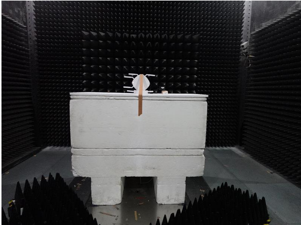
03CH02-HY Radio 2 Dipole Antenna (2T2S)
