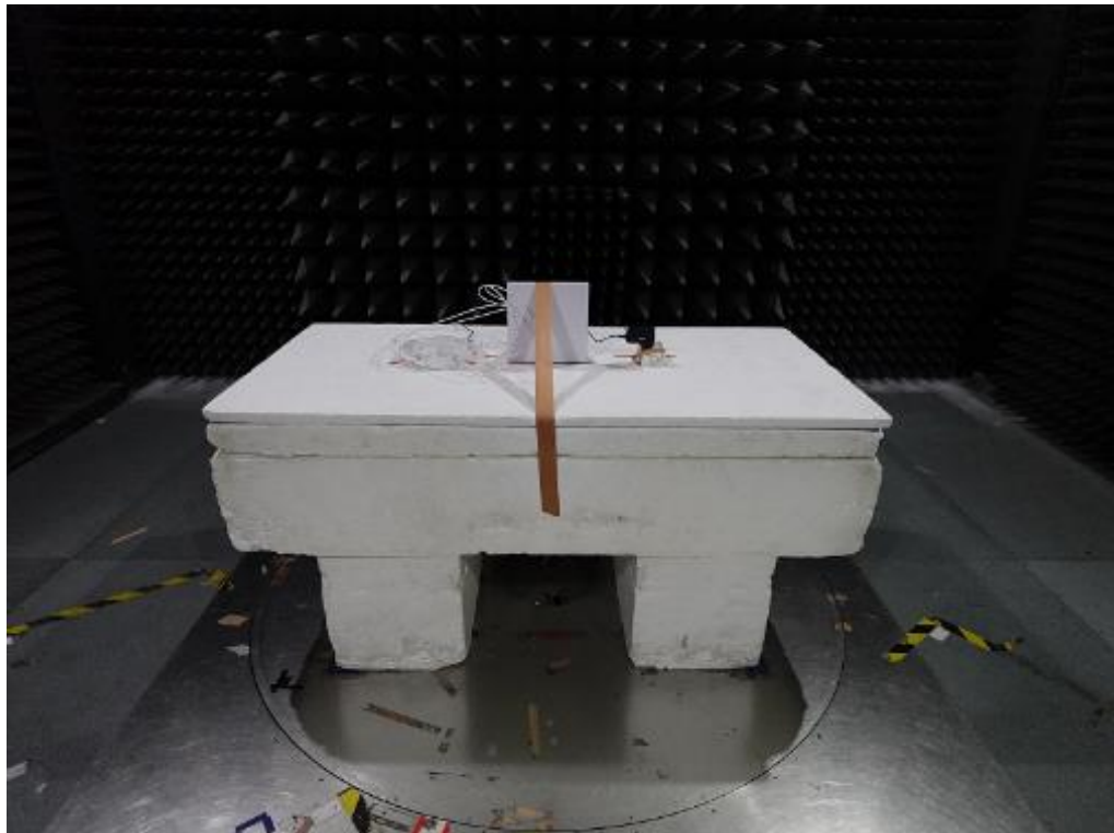
Radio 3 Dual-Polarized MIMO Panel Antenna (2T2S)
