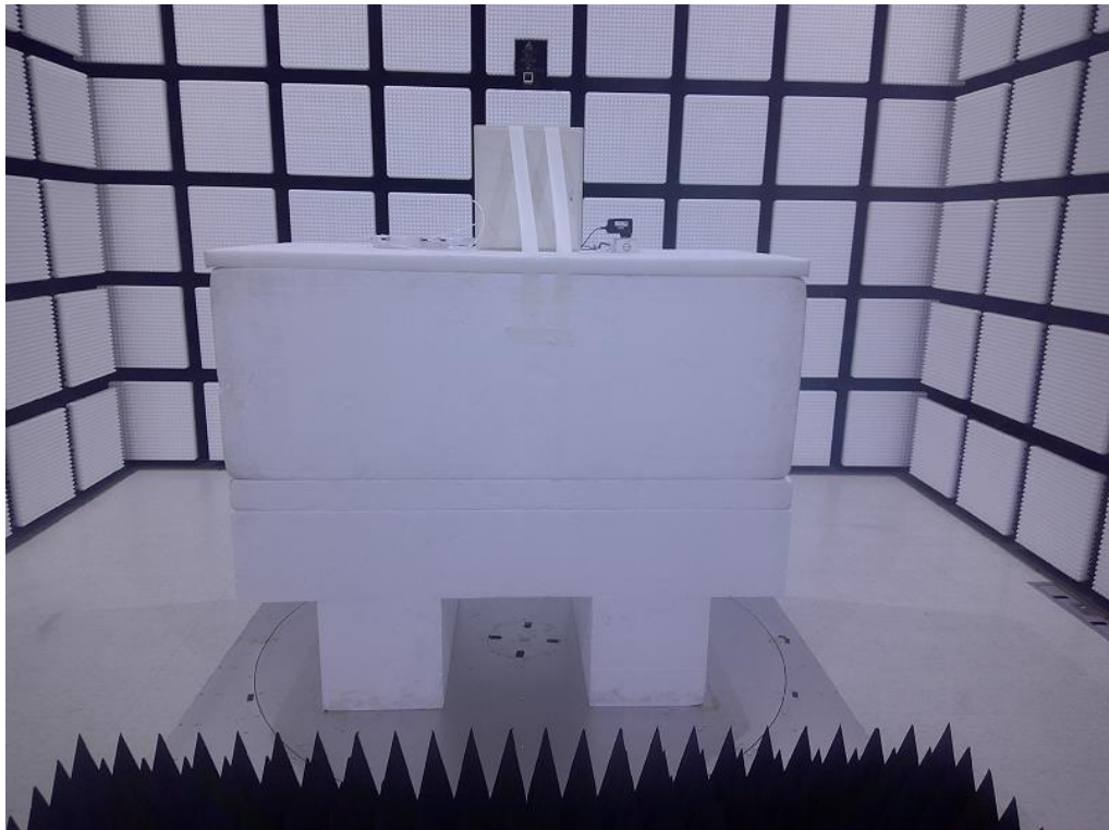
Radio 3 MIMO-directional Antenna (2T1S) and 2T2S
