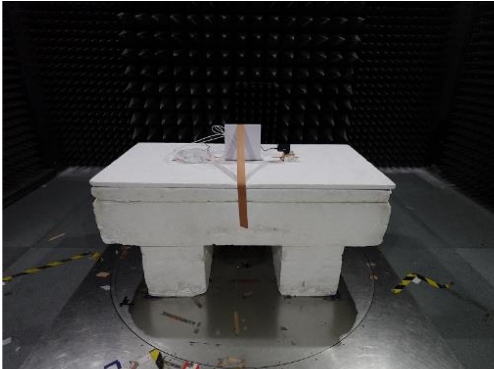
Radio 2 Dual-Polarized MIMO Panel Antenna (1T1S)
