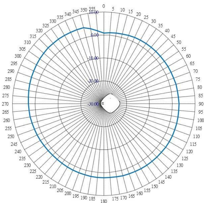
Figure 14: AP4020 2GHz Sensor Horizontal Radiation Pattern
