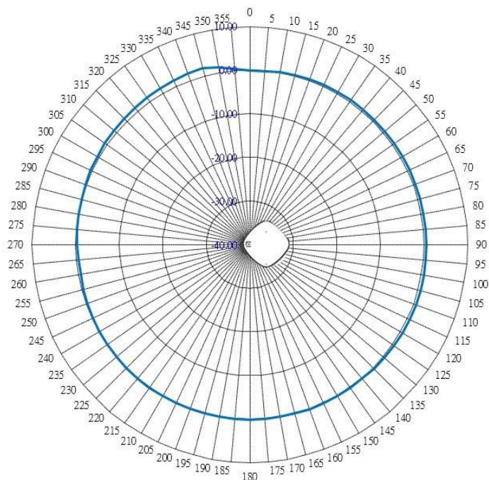
Figure 5: AP4020 5 GHz Low Horizontal Radiation Pattern
