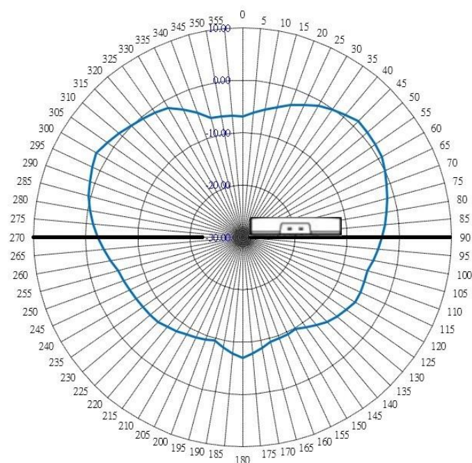
Figure 13: AP4020 2GHz Sensor Vertical Radiation Pattern
