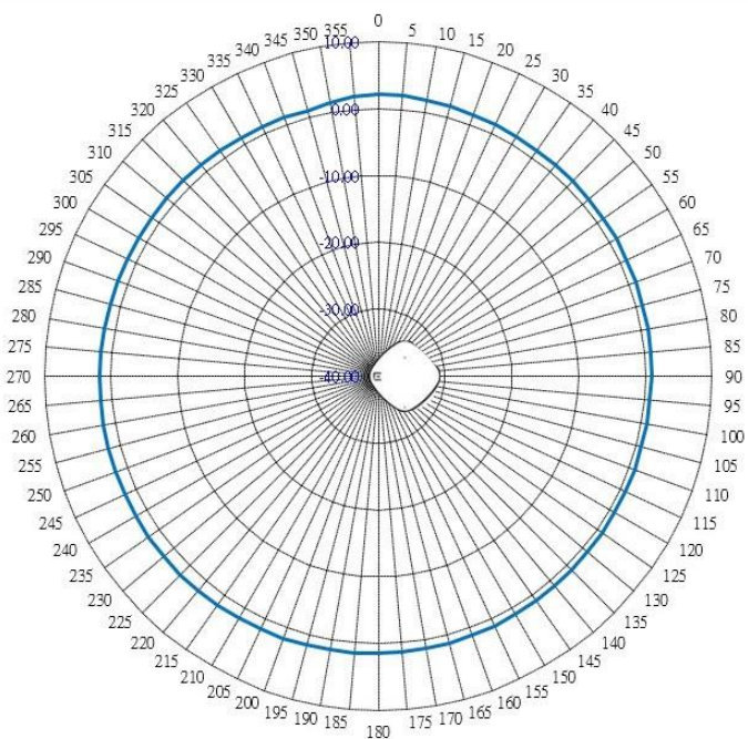
Figure 16: AP4020 5GHz Sensor Horizontal Radiation Pattern
