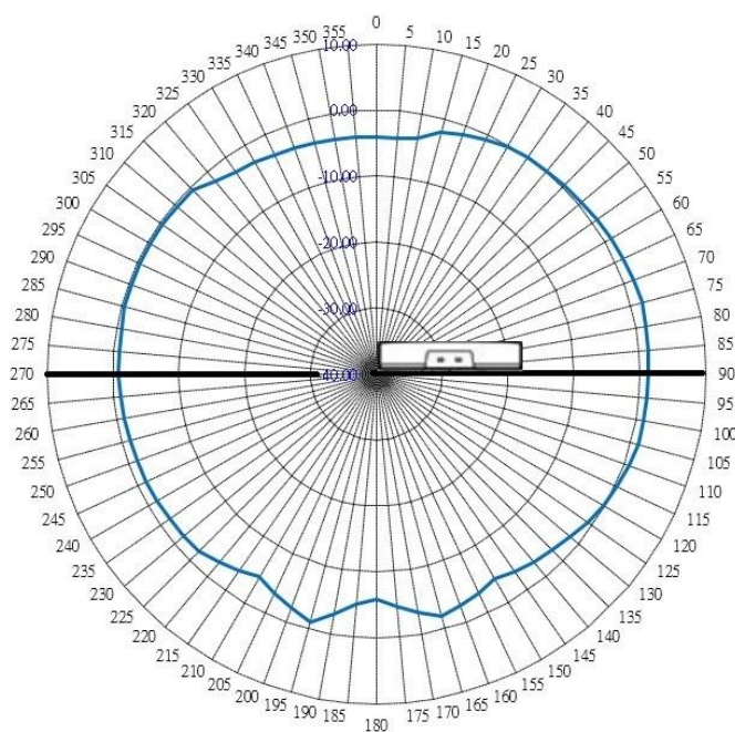
Figure 1: AP4020 2GHz Vertical Radiation Pattern
