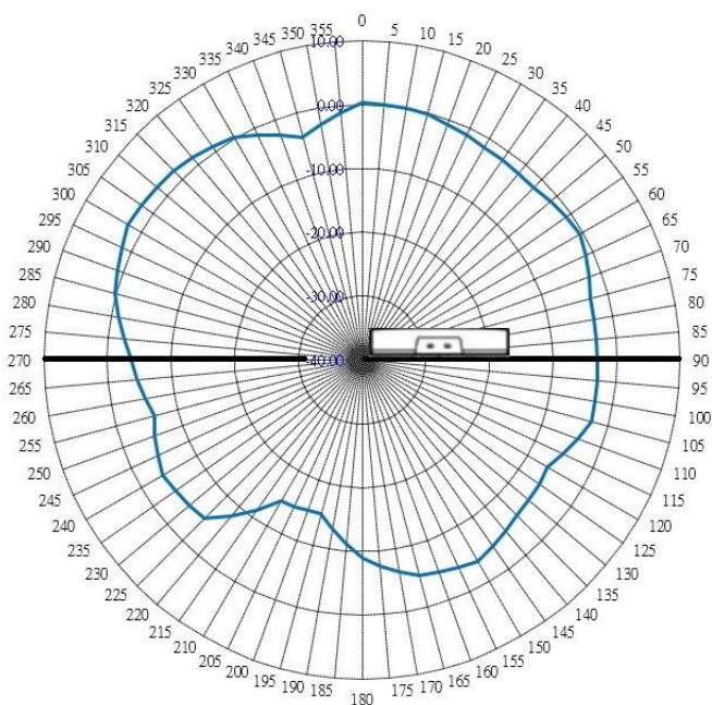
Figure 9: AP4020 BLE Radio 1 Vertical Radiation Pattern
