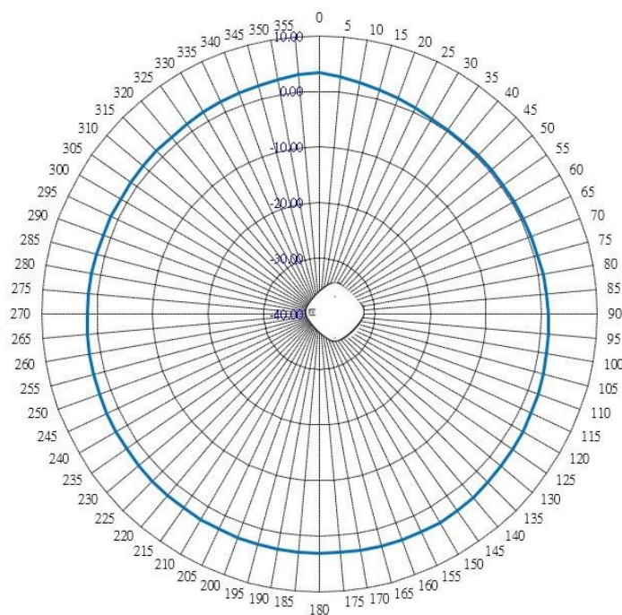
Figure 6: AP4020 5 GHz Horizontal Radiation Pattern
