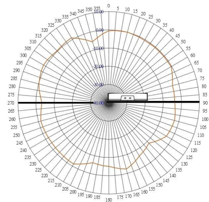
Figure 11: AP4020 BLE Radio 2 Vertical Radiation Pattern
