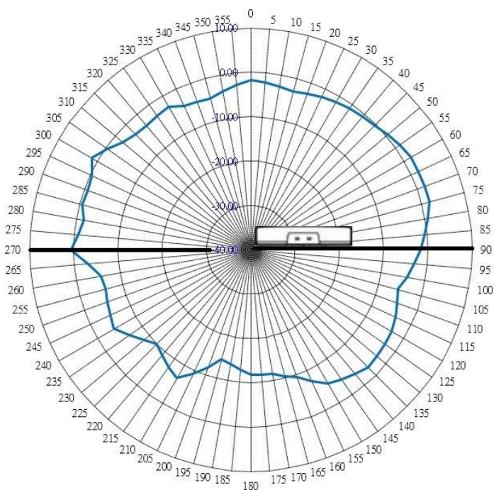
Figure 7: AP4020 6 GHz Vertical Radiation Pattern
