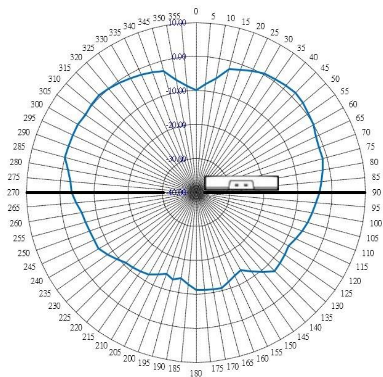
Figure 3: AP4020 5 GHz Low Vertical Radiation Pattern
