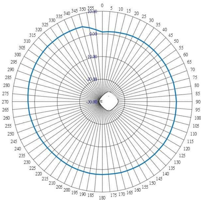
Figure 14: AP4020X 2GHz Sensor Horizontal Radiation Pattern
