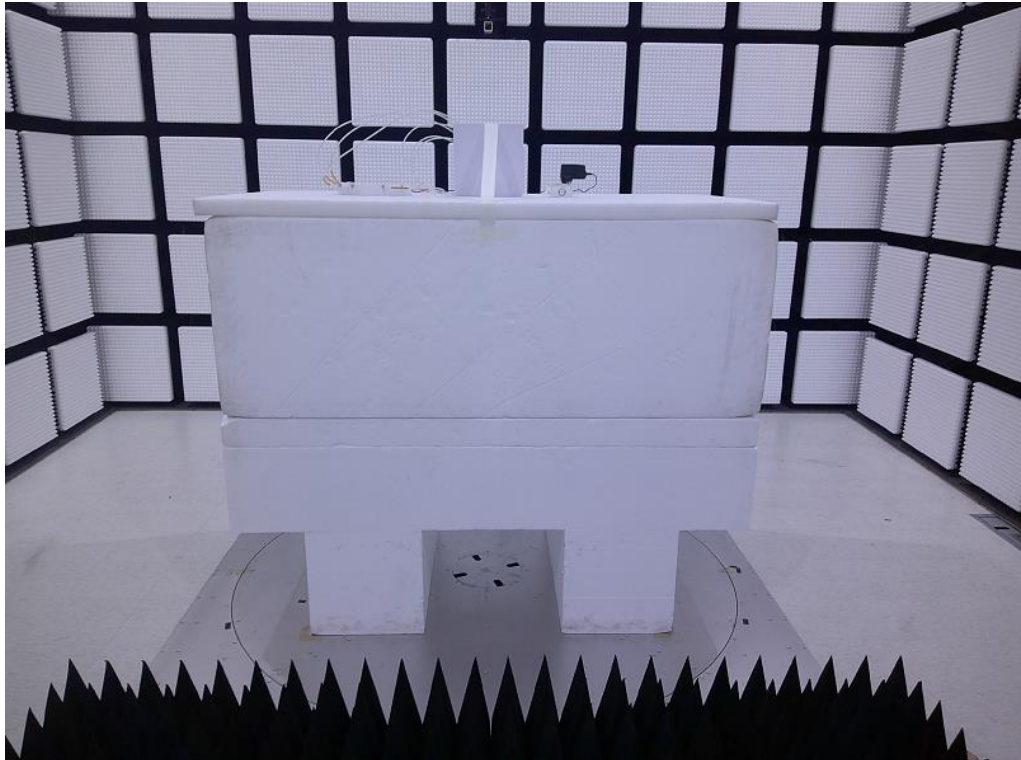
Radio 1 Dual-Polarized MIMO Panel Antenna (1T1T&2T2S)
