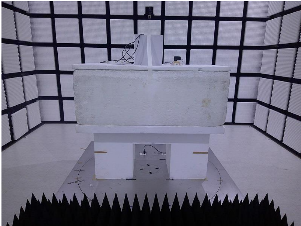
Beamforming Panel Antenna
