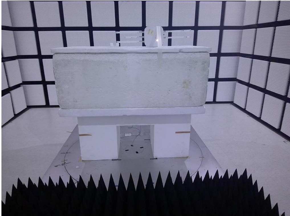
Radio 1_Dipole 2T1S, 2T2S
