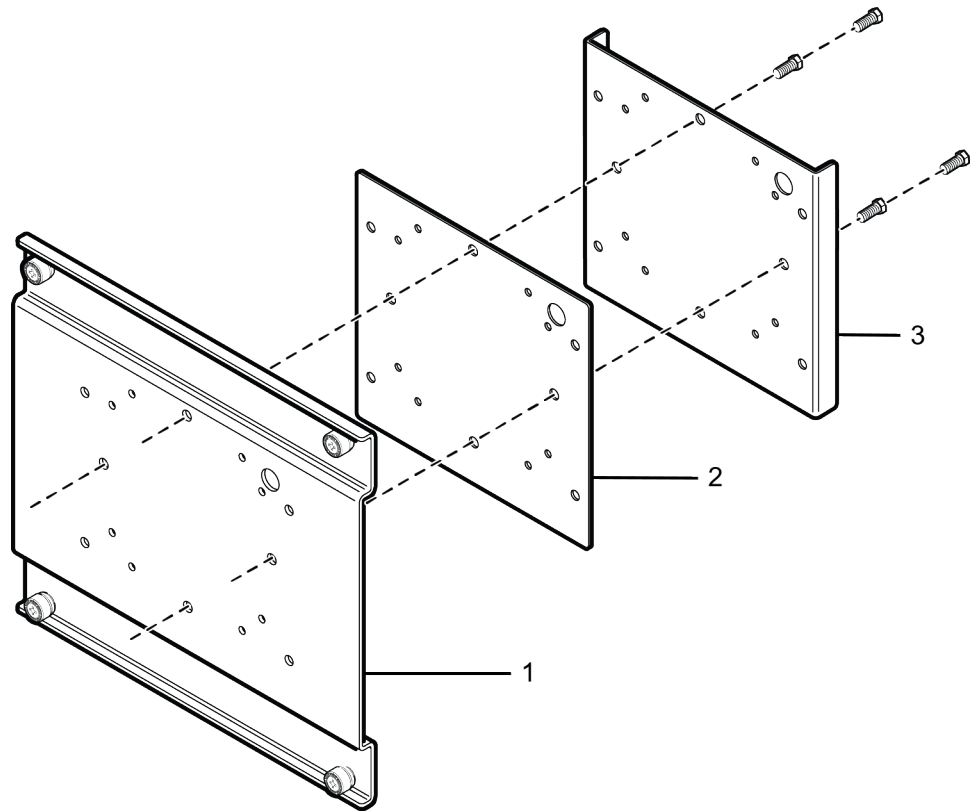
Figure 10: VMM access point attach assembly plate stiffener 1 and stiffener 2
