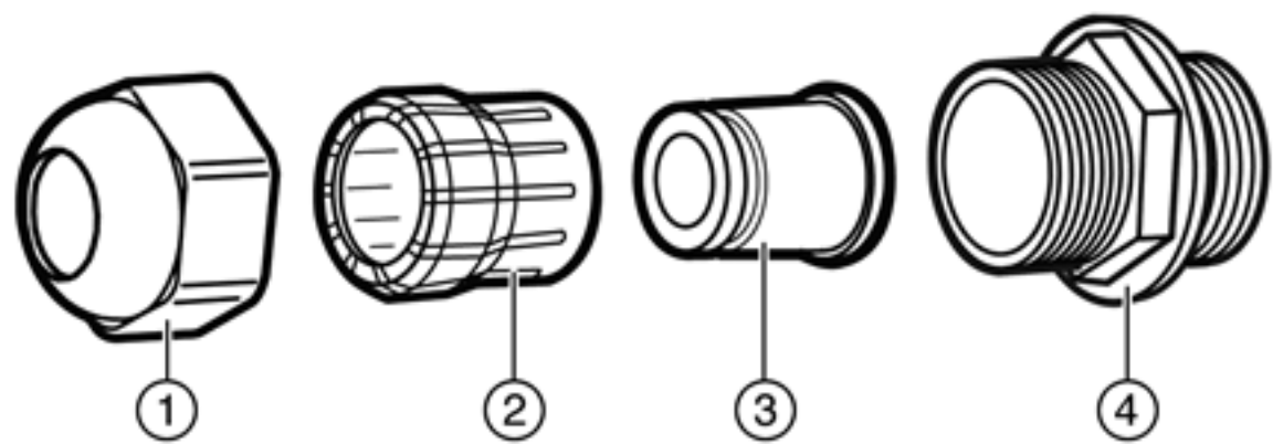
Figure 19: RJ45 cable gland adapter assembly
