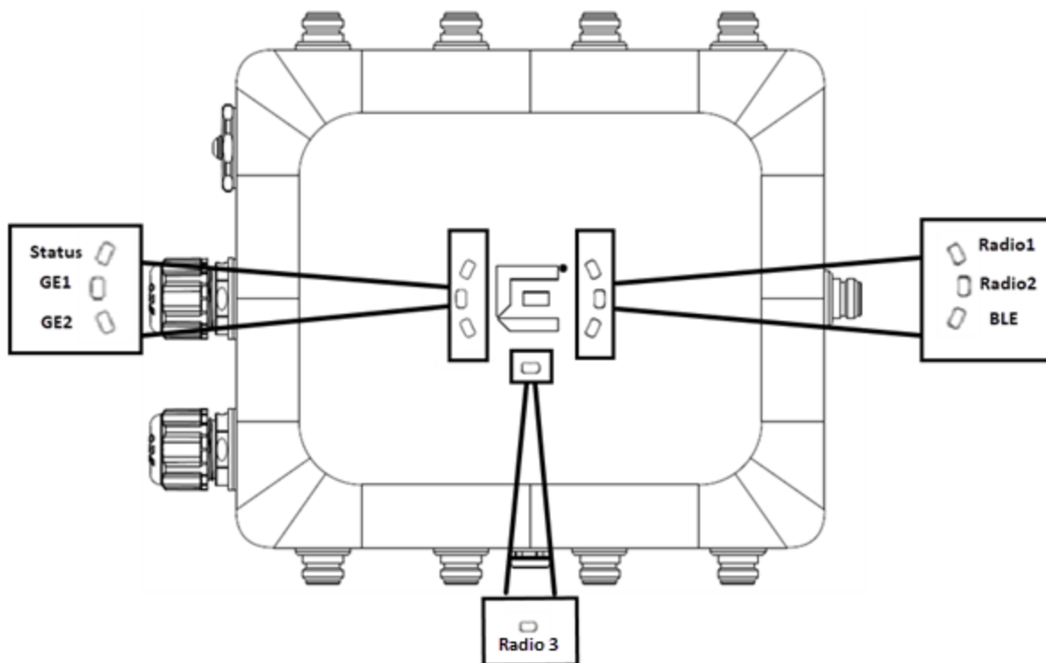
Figure 3: AP460i/e LED indicators
