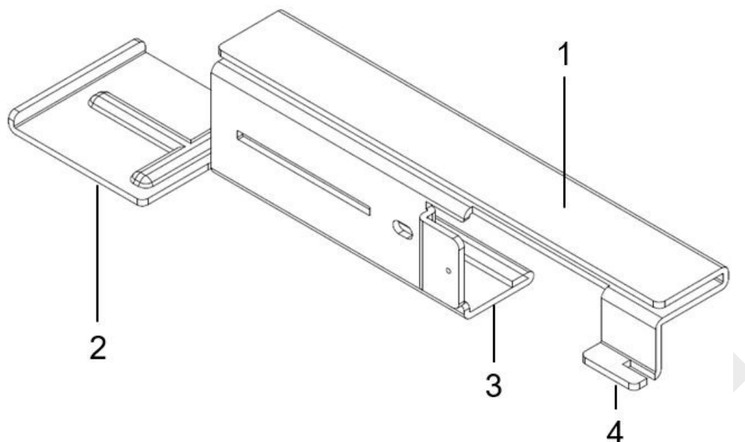
Figure 17: ACC-BKT-TB-NF adapter
