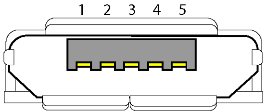
Figure 8: Micro-B model Console Port Pin Information
