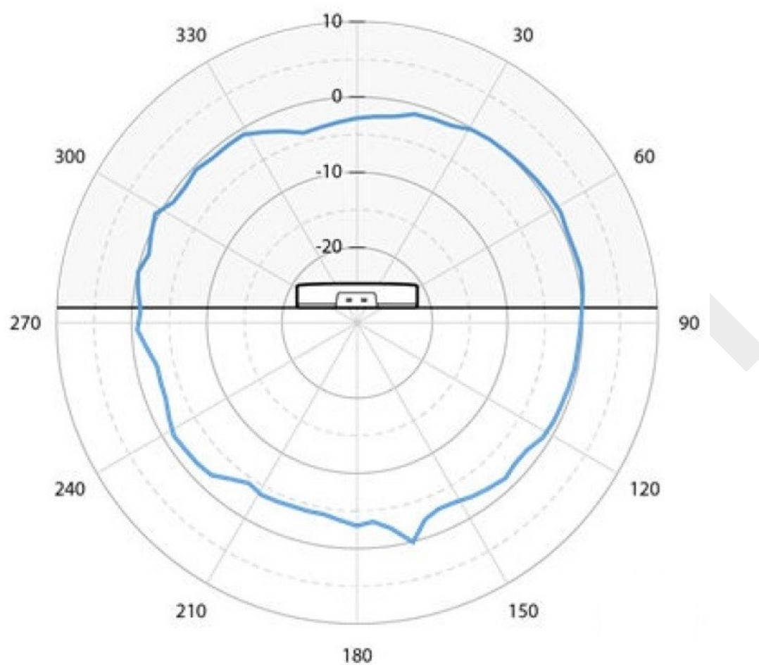
AP5020 2GHz Vertical Radiation Pattern
