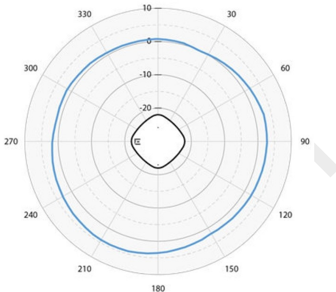
Figure 5: AP5020 5 GHz Horizontal Radiation Pattern
