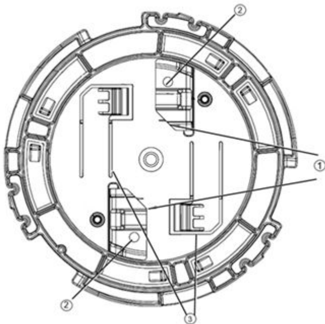
Figure 10: AH-ACC-BKT-AX-TB bracket
