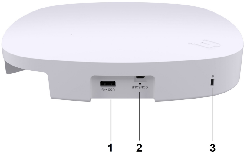
Figure 1: AP5020 Front Hardware Ports and Connections
