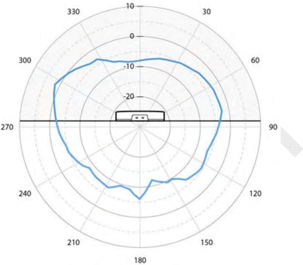
Figure 6: AP5020 6 GHz Vertical Radiation Pattern
