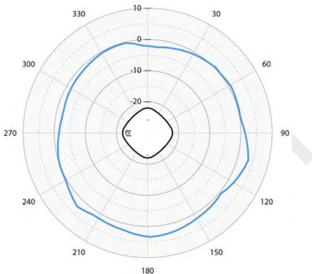
Figure 7: AP5020 6 GHz Horizontal Radiation Pattern
