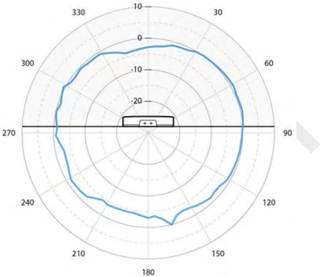
AP5020 2GHz Vertical Radiation Pattern
