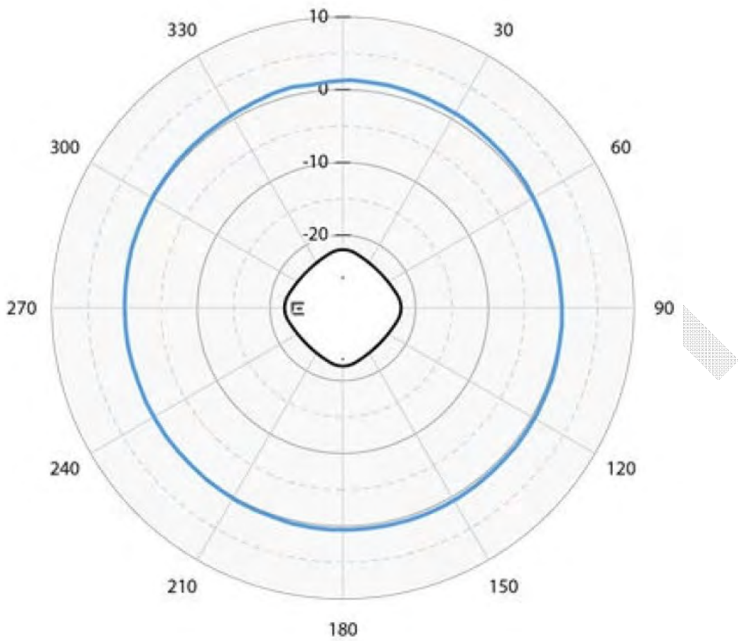
Figure 3: AP5020 2GHz Horizontal Radiation Pattern
