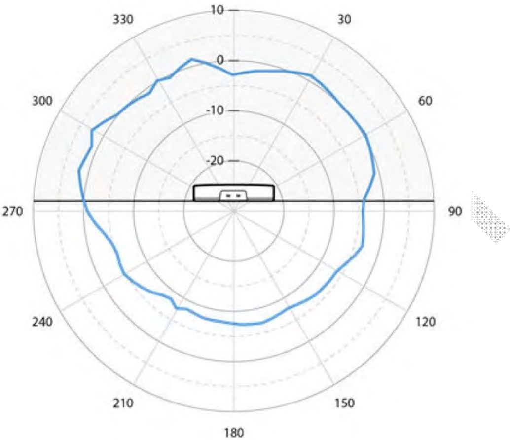
Figure 4: AP5020 5 GHz Vertical Radiation Pattern
