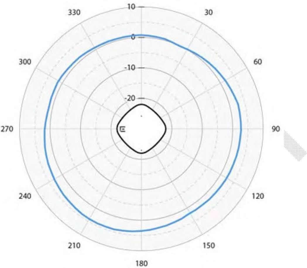
Figure 5: AP5020 5 GHz Horizontal Radiation Pattern
