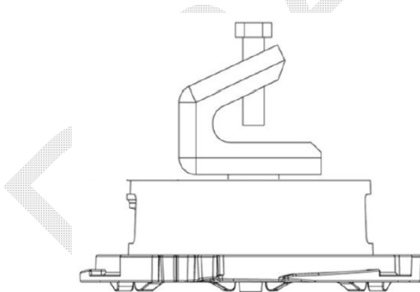
Figure 21: ACC-BKT-AX-BEAM accessory bracket
