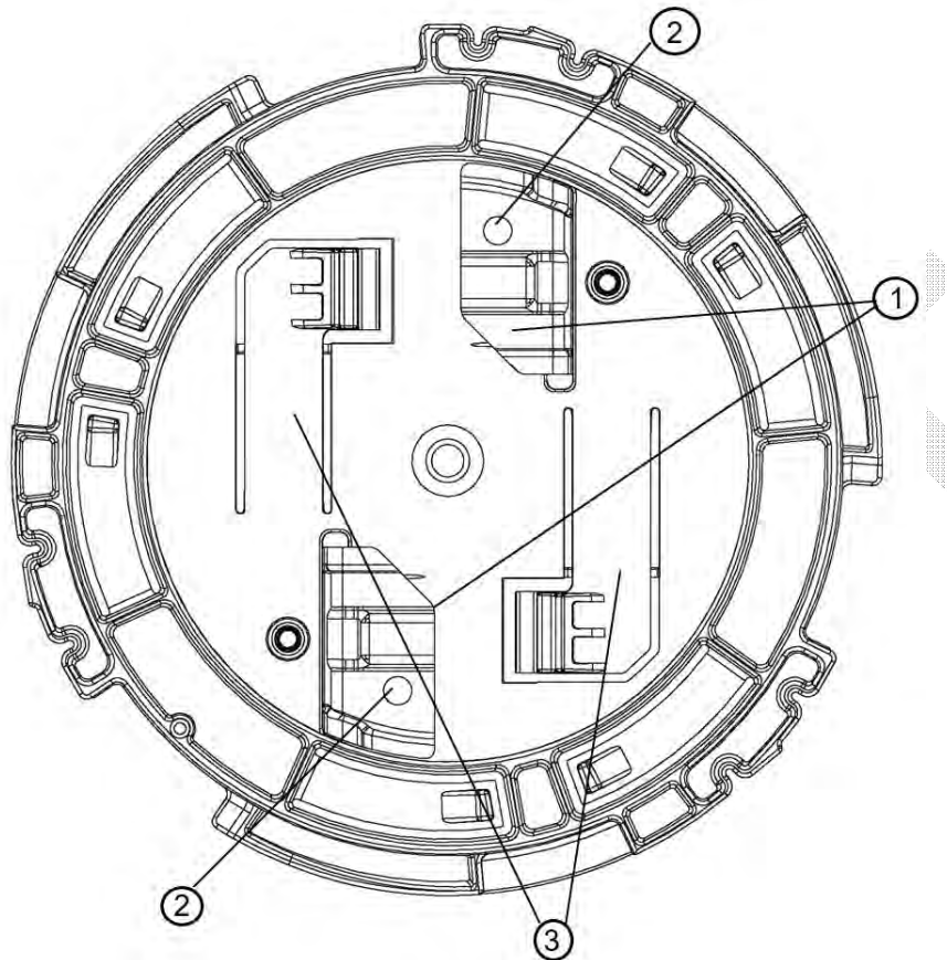
Figure 18: AH-ACC-BKT-AX-TB accessory bracket
