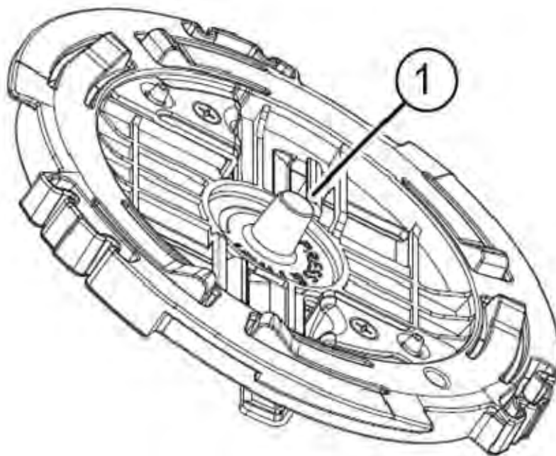
Figure 13: AH-ACC-BKT-AX-SL accessory bracket circular tip
