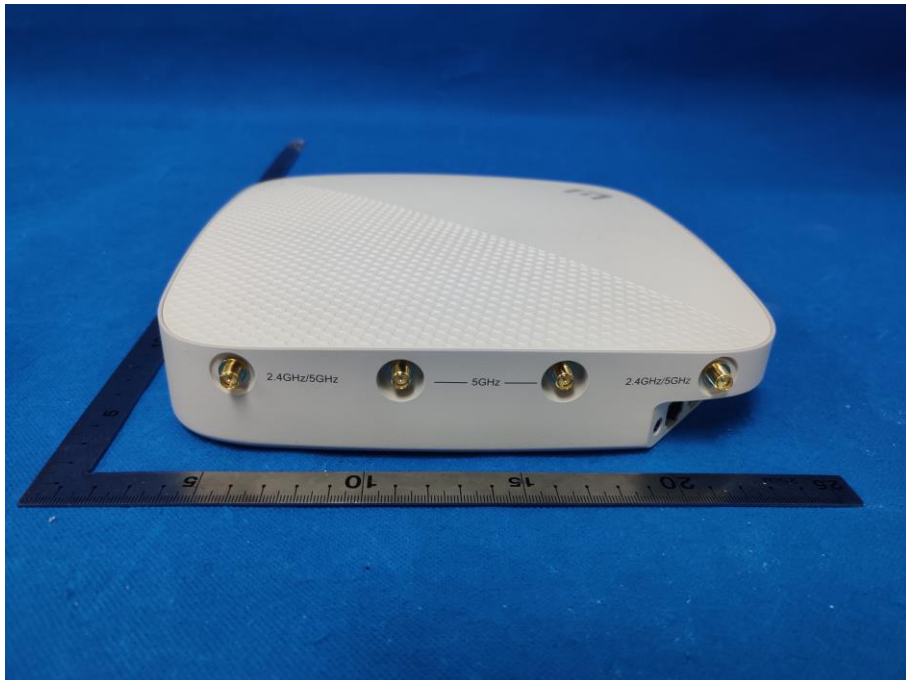
(2) EUT Photo (AP510CX)
