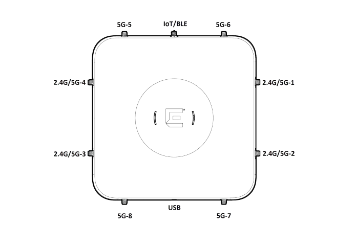
Figure 3 AP510e External RP-SMA Antenna Connectors
