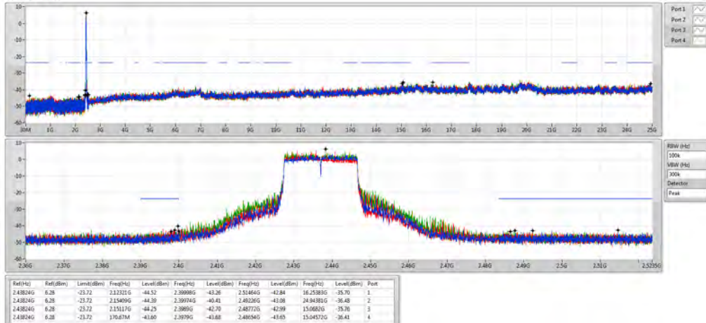
802.11ax HEW20_Nss1,(MCS0)_4TX 2437MHz
