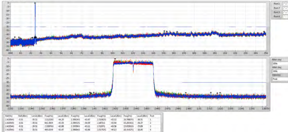
802.11ax HEW40_Nss1,(MCS0)_4TX 2437MHz
