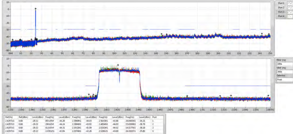
802.11ax HEW40_Nss4,(MCS0)_4TX 2422MHz
