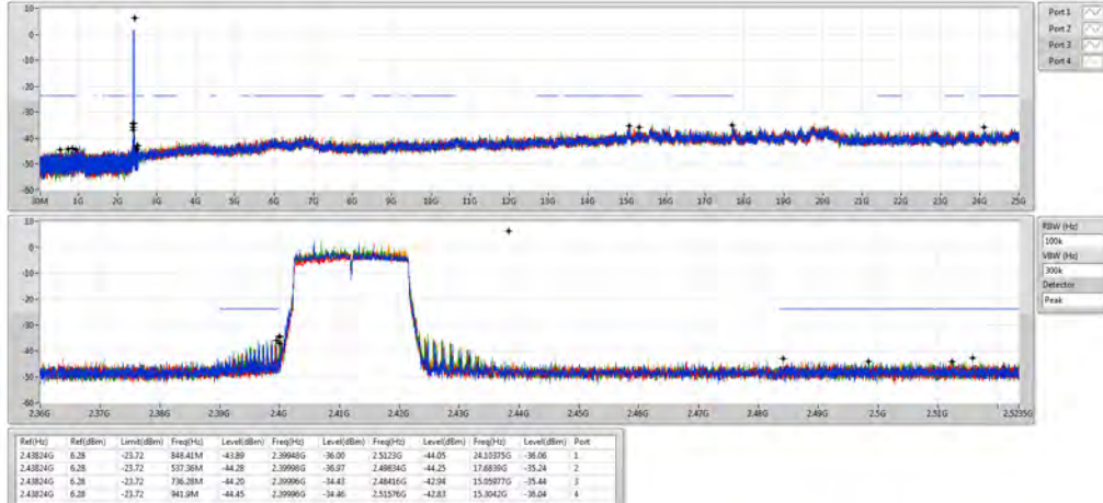
802.11ax HEW20_Nss1,(MCS0)_4TX 2412MHz
