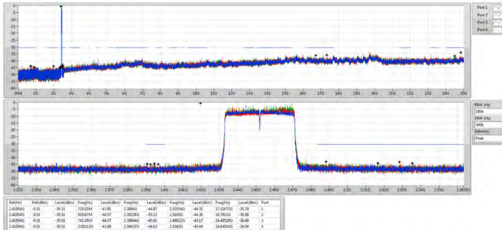
802.11ax HEW40_Nss1,(MCS0)_4TX 2452MHz
