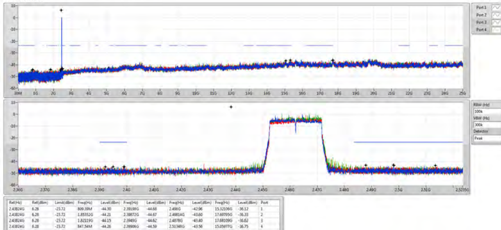
802.11ax HEW20_Nss1,(MCS0)_4TX 2462MHz
