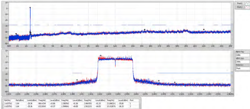
802.11ax HEW40_Nss2,(MCS0)_2TX
