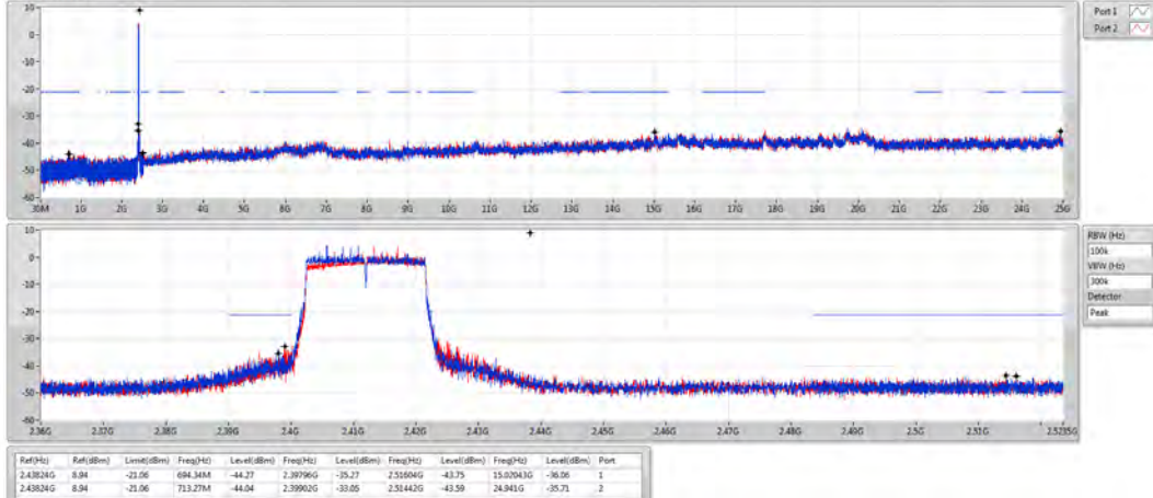
802.11ax HEW20_Nss2,(MCS0)_2TX
