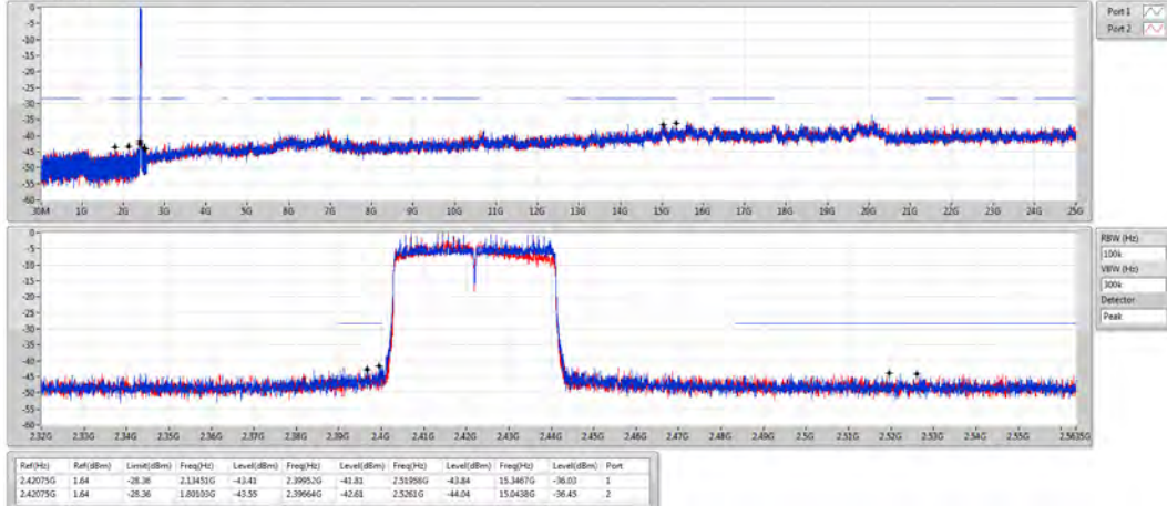
802.11ax HEW40_Nss2,(MCS0)_2TX
