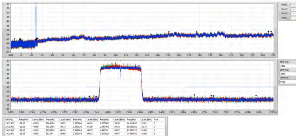
802.11ax HEW40-BF_Nss1,(MCS0)_4TX 2422MHz
