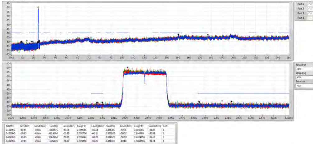
802.11ax HEW40-BF_Nss1,(MCS0)_4TX 2437MHz
