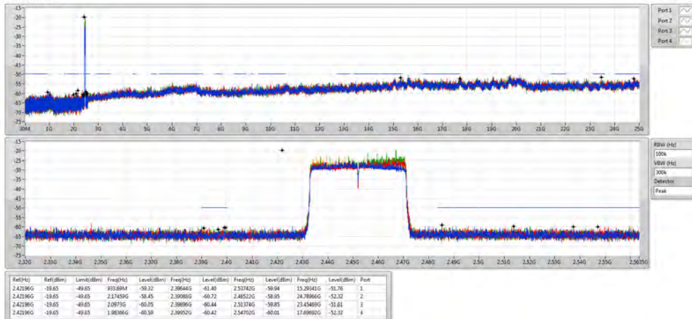
802.11ax HEW40-BF_Nss1,(MCS0)_4TX 2452MHz
