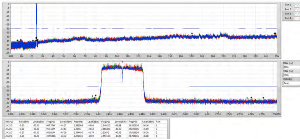
802.11ax HEW40_Nss4,(MCS0)_4TX 2422MHz
