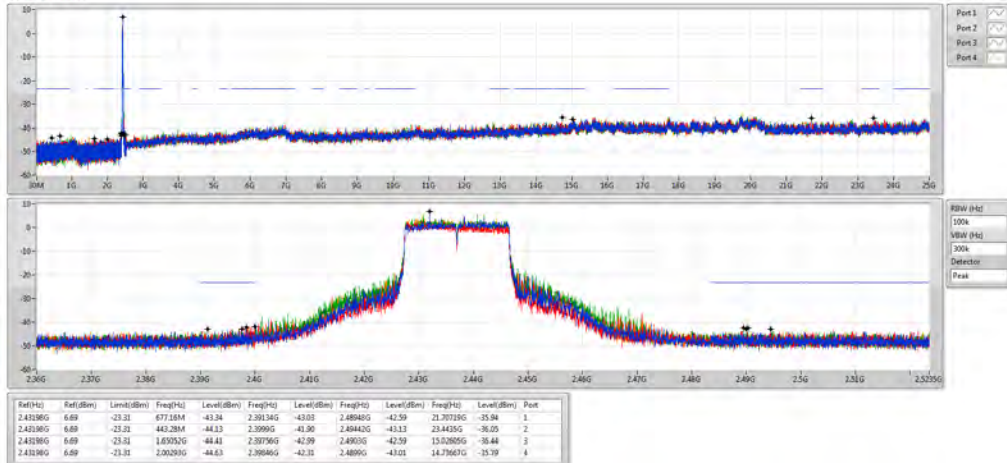
802.11ax HEW20_Nss1,(MCS0)_4TX 2437MHz
