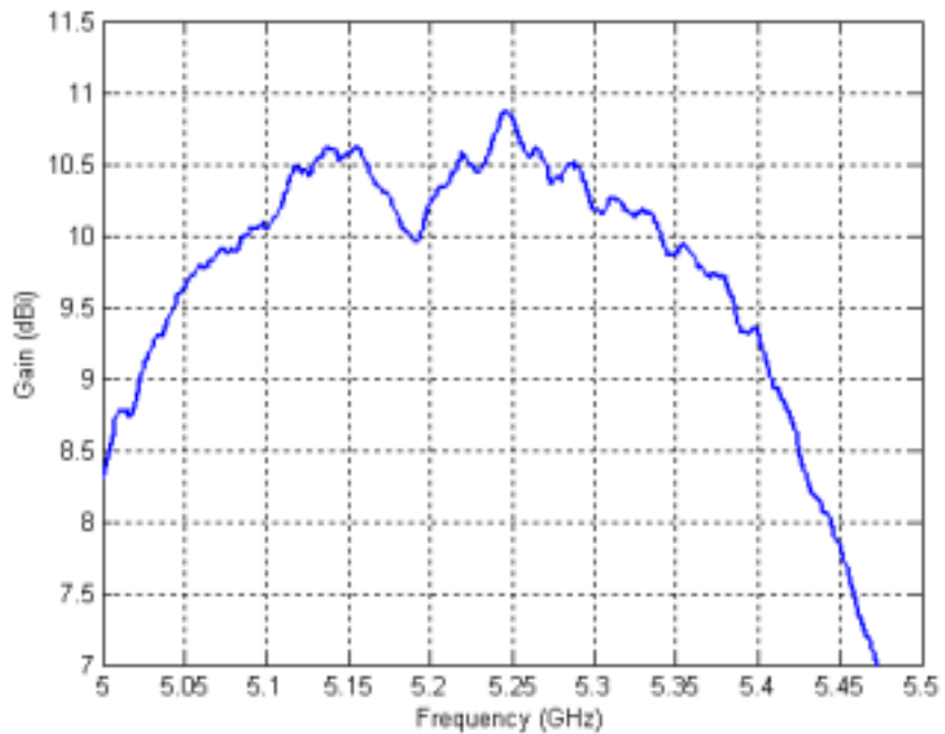
Radiating Element Average Gain
