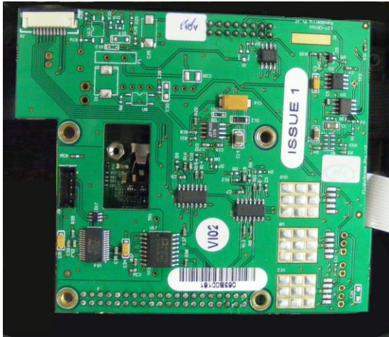
Interface PCB (top)
