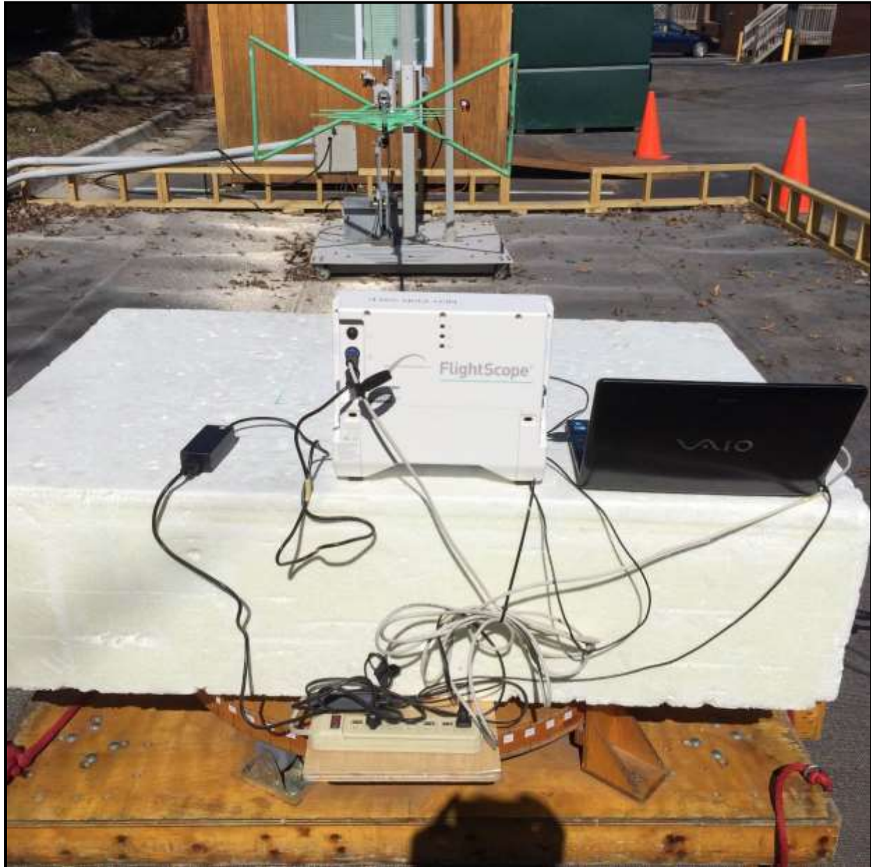
Photograph 2: Radiated Emissions - Rear View
