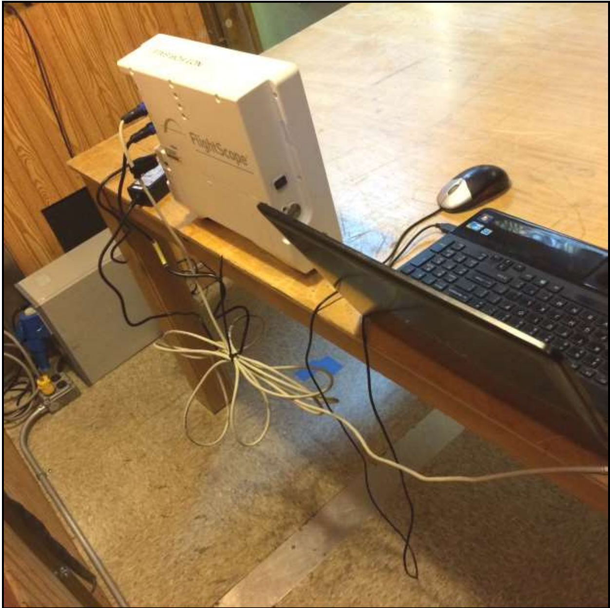
Photograph 4: Conducted Emissions - Rear View
