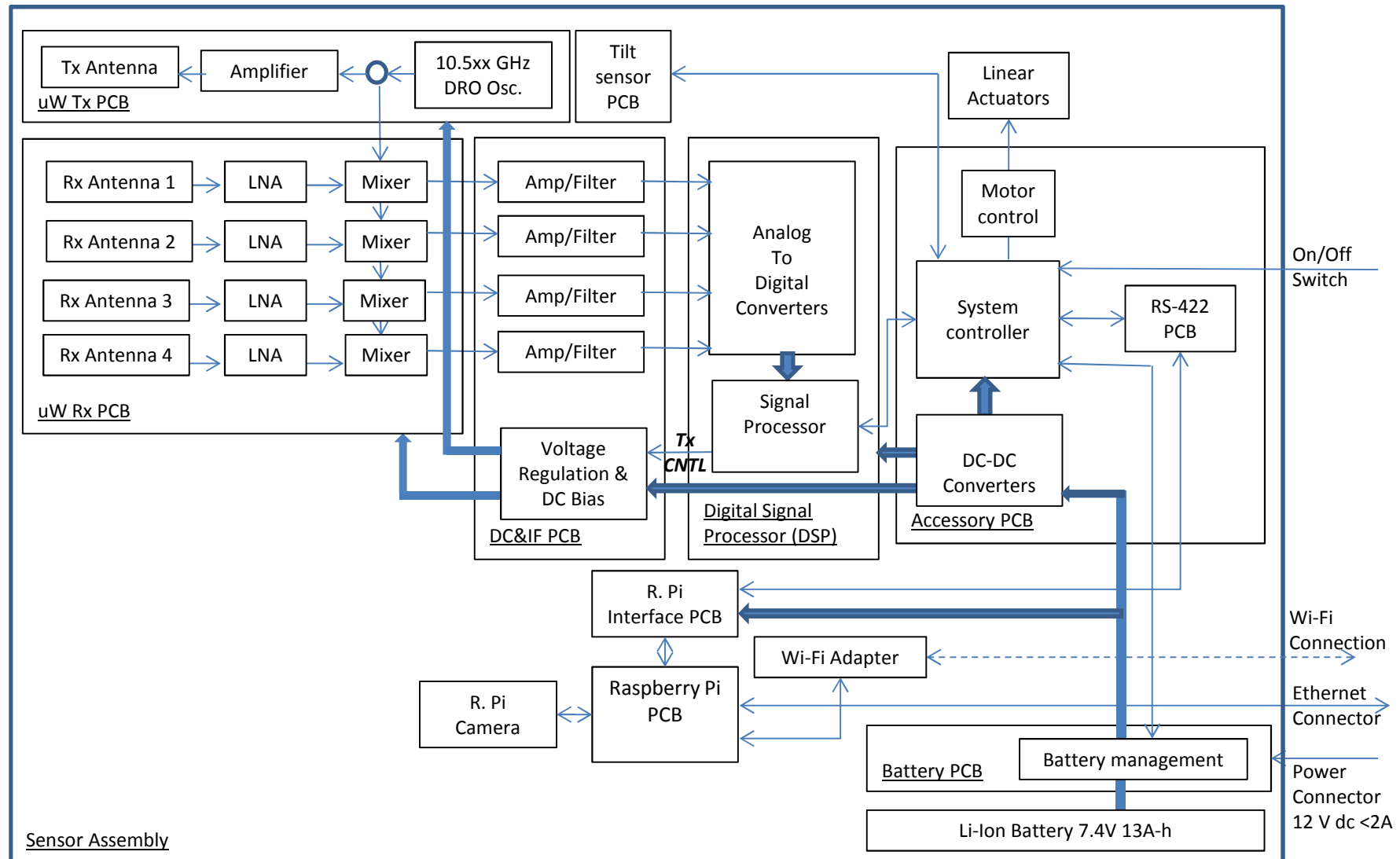
FlightScope X2 Elite System Block Diagram Part No E51-HP244 Ver A; 5 Dec 2014
