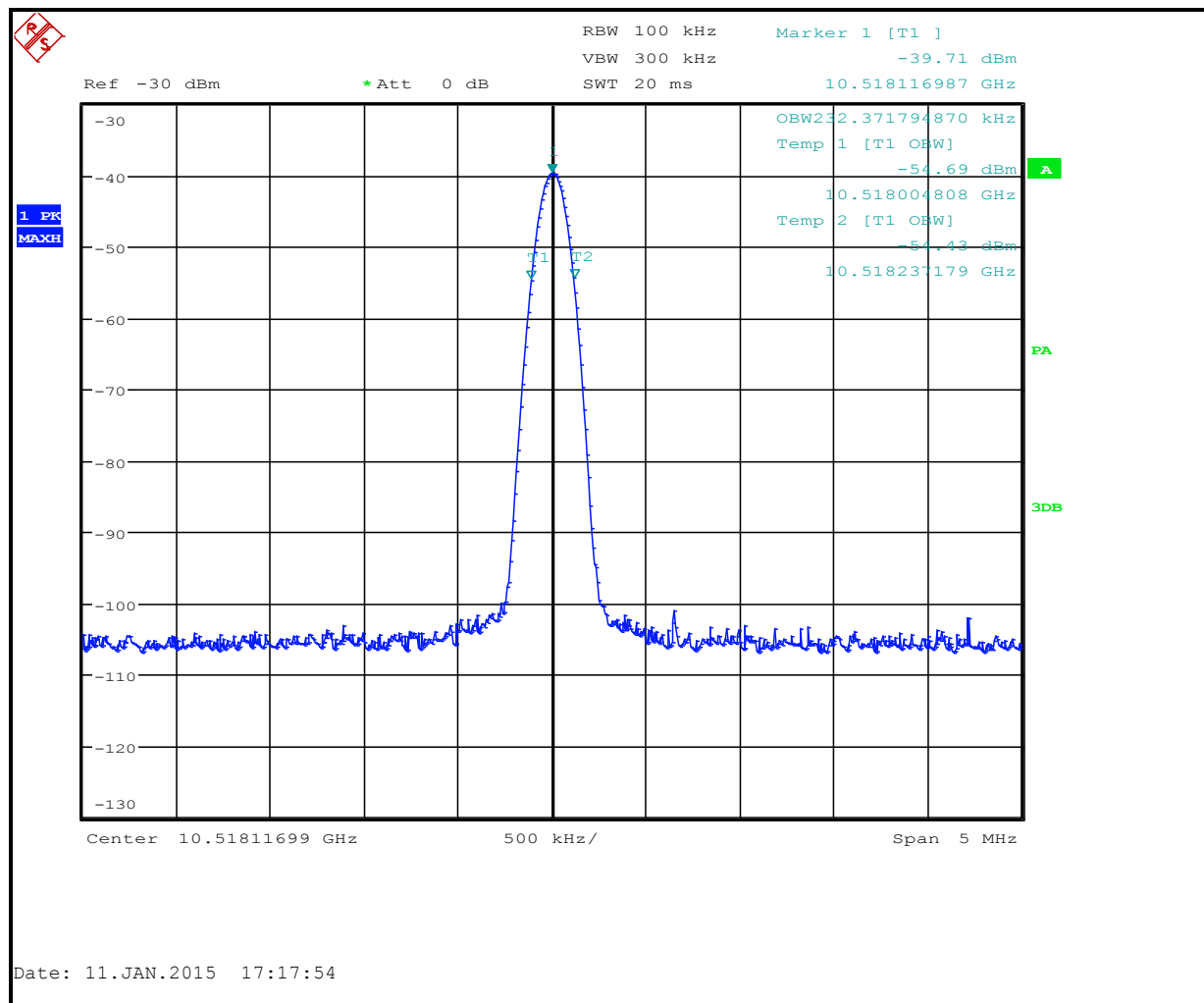
Plot 5-1: 99% Bandwidth
