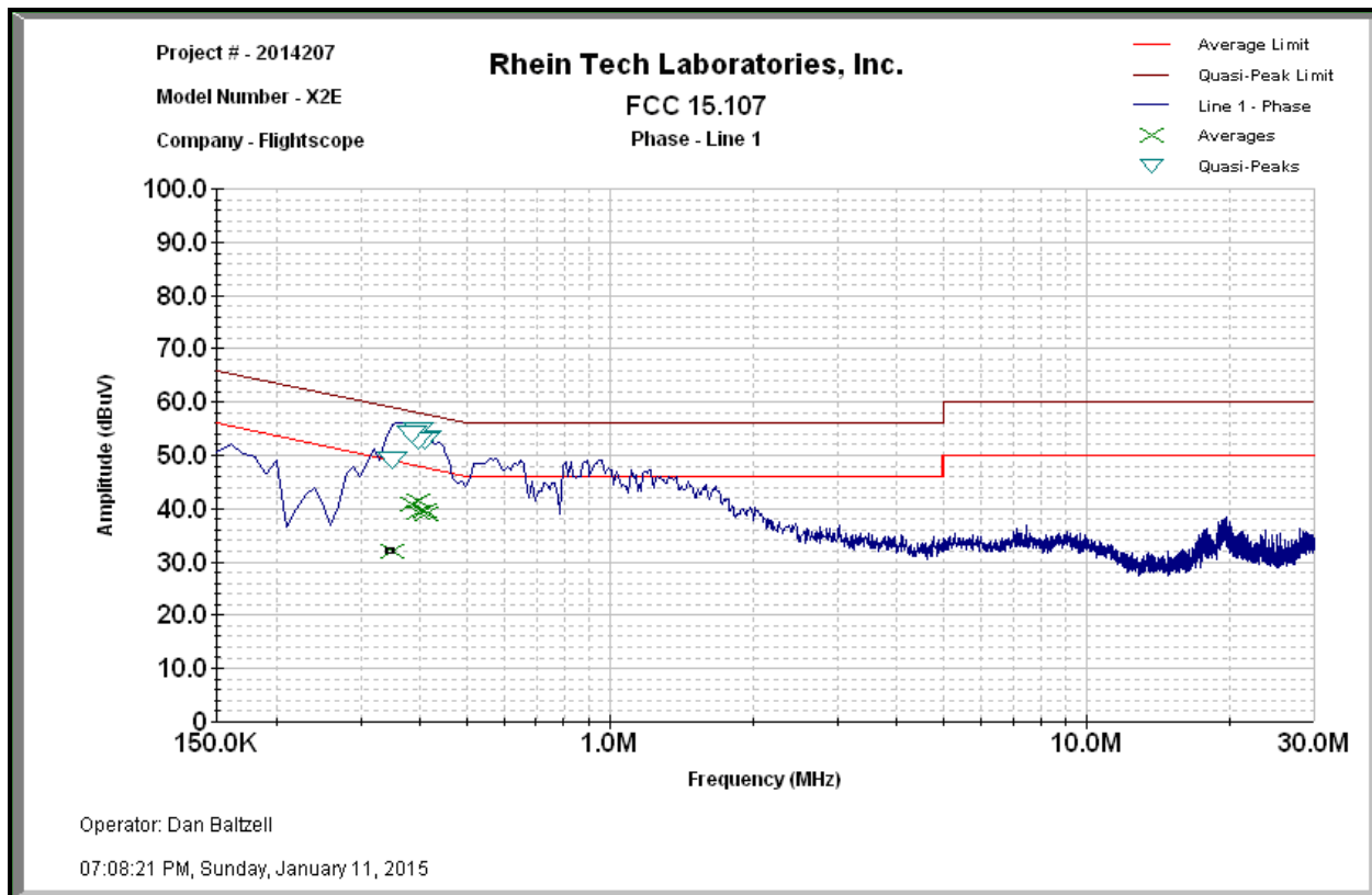
Plot 4-1: Conducted Emissions (Phase Side)
