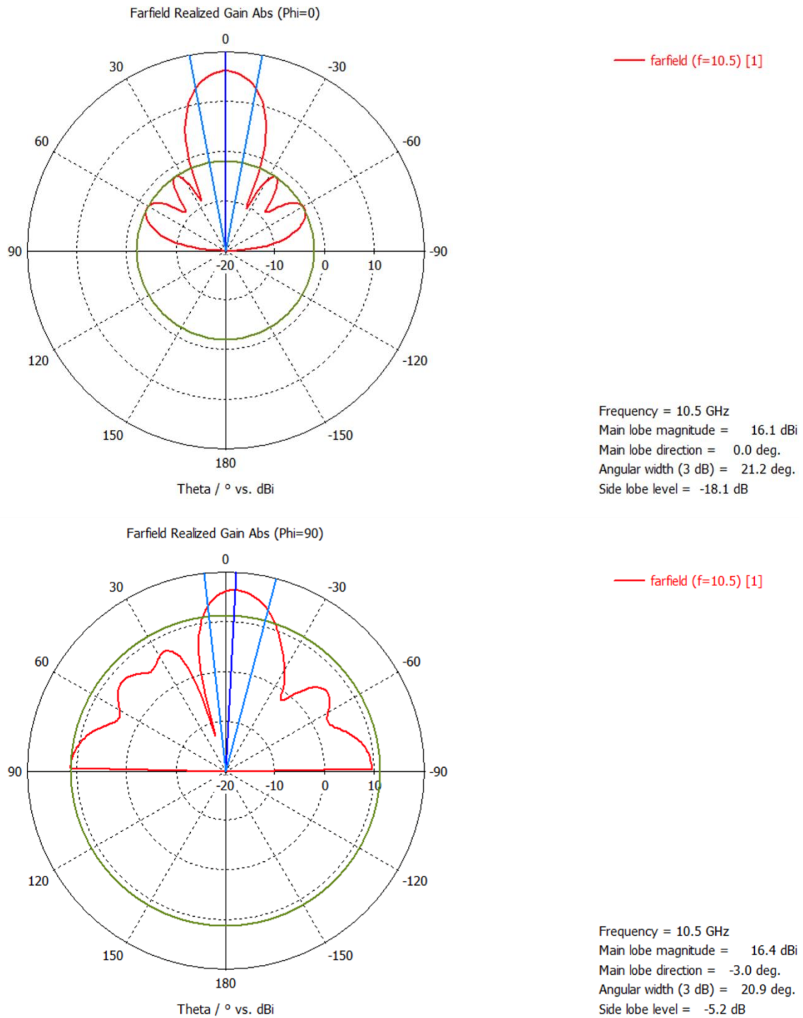
Figure 2 Antenna Gain
