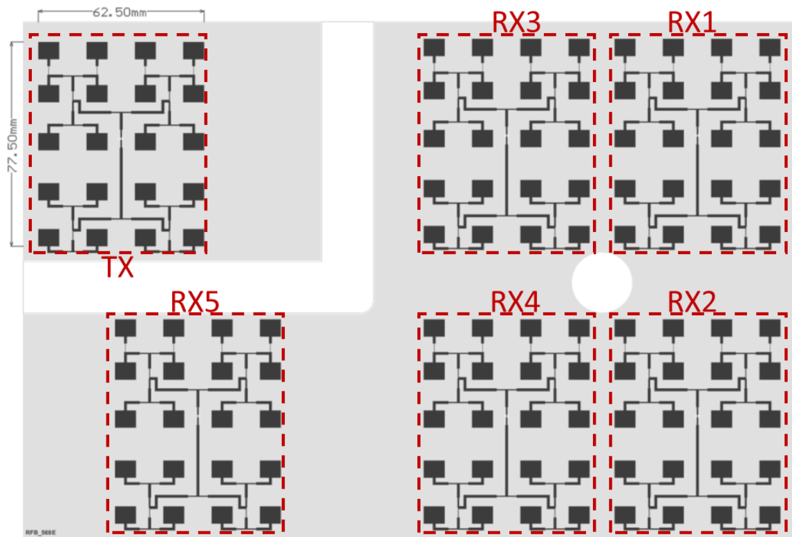
Figure 3 Antenna patches
