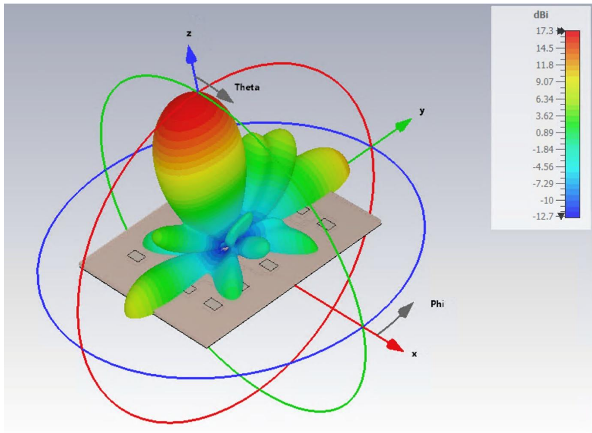
Figure 1 3D Antenna Radiation Pattern
