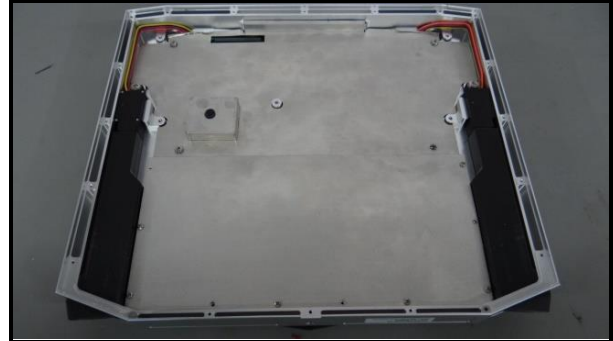
Internal Assembly without DC/IF PCB assembly and with internal electronics shield
