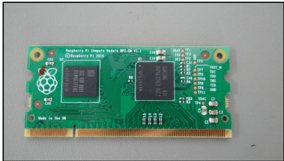
Raspberry Pi Compute Module Top
