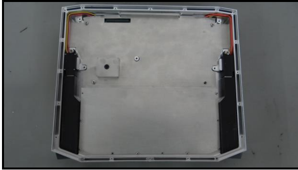
Internal Assembly without DC/IF PCB assembly and with internal electronics shield
