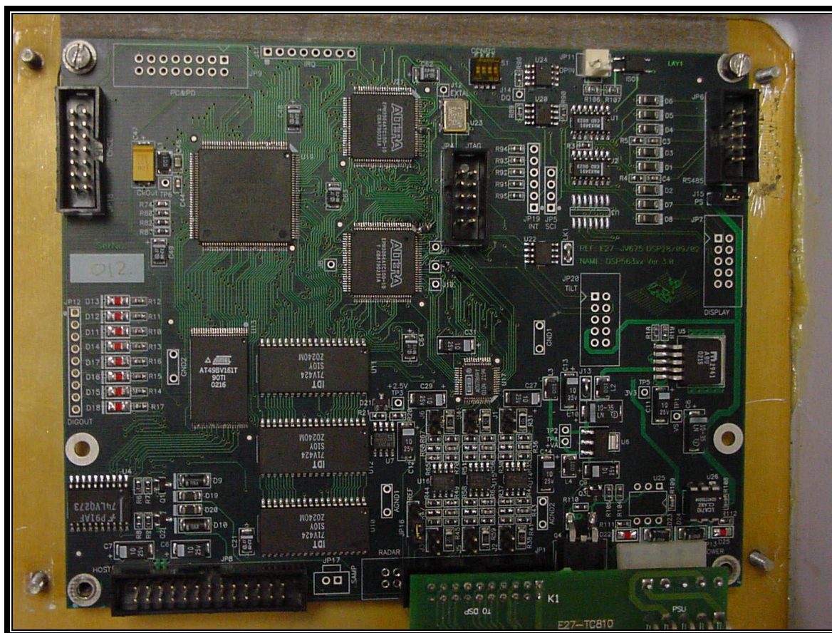
PHOTOGRAPH 12: DSP PCB TOP
