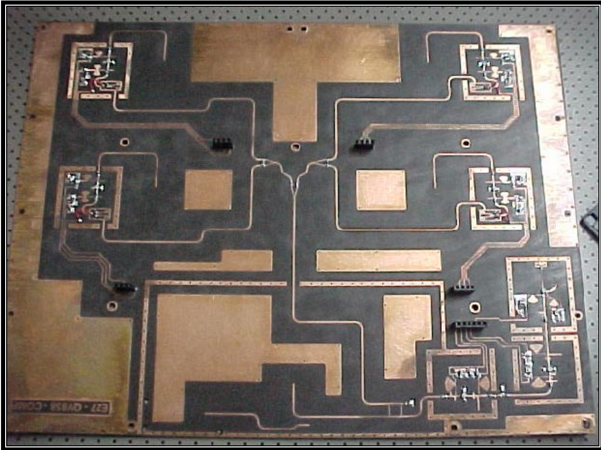
PHOTOGRAPH 16: ANTENNA WITHOUT SHIELDS
