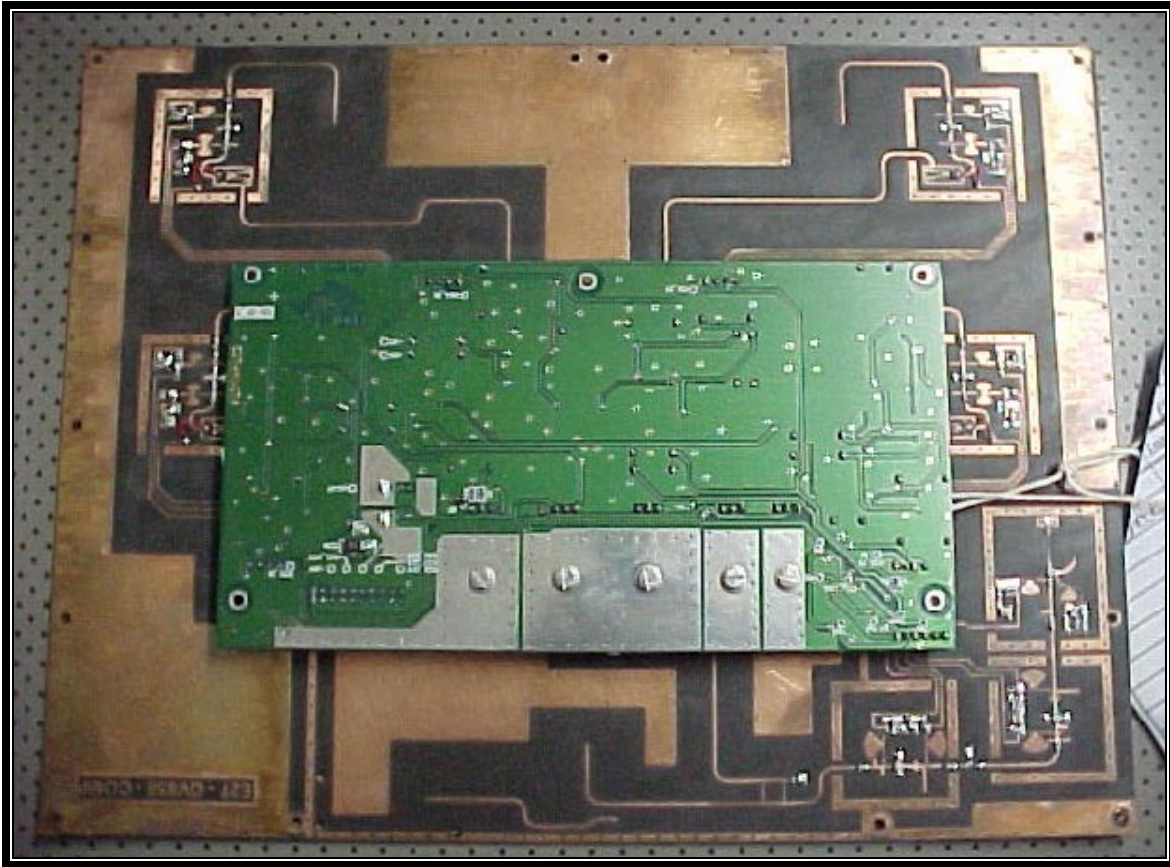
PHOTOGRAPH 14: ANTENNA AND DC/VIDEO BOARD
