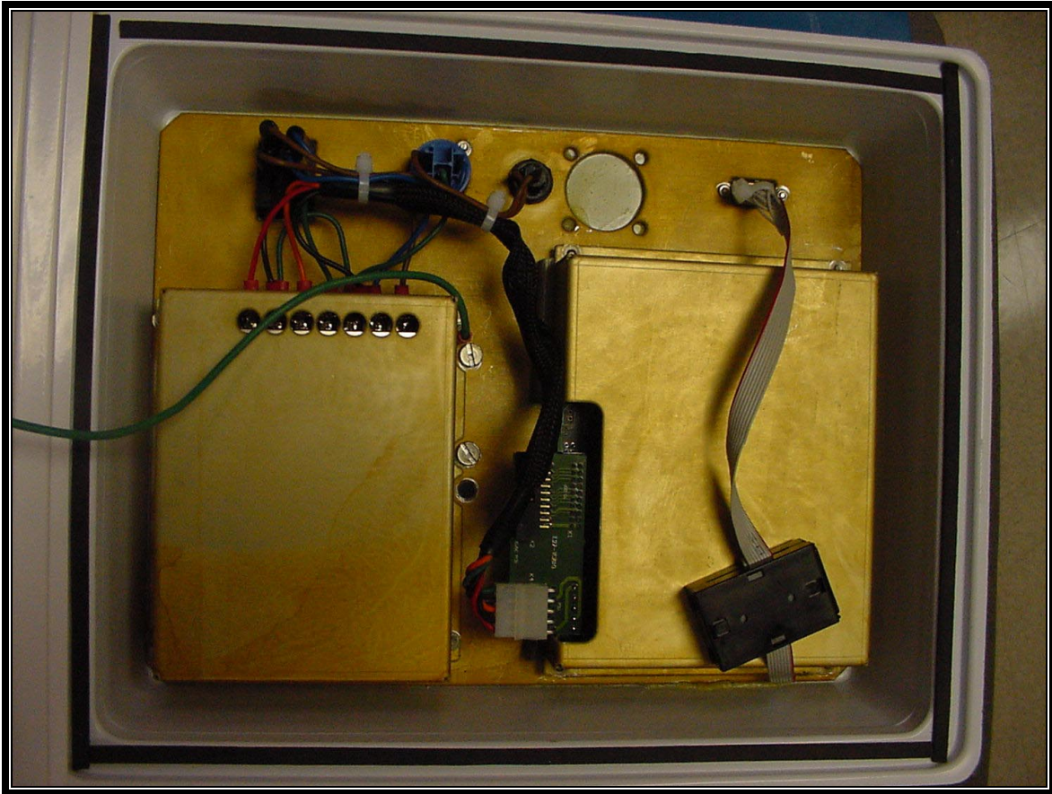
PHOTOGRAPH 10: DSP AND POWER SUPPLY WITH SHIELDS
