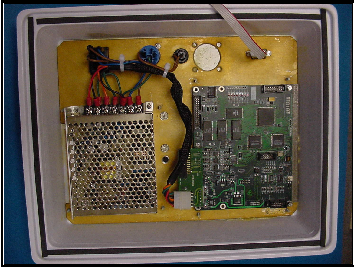
PHOTOGRAPH 11: DSP AND POWER SUPPLY WITHOUT SHIELDS
