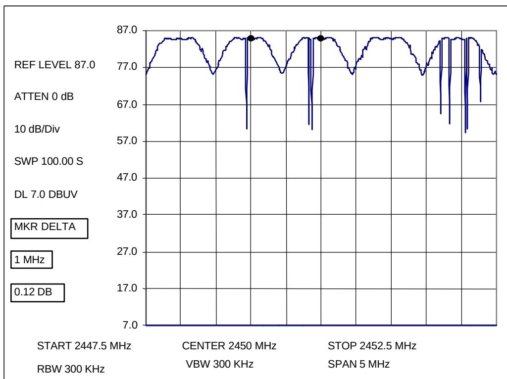
Plot 2: Channel spacing
