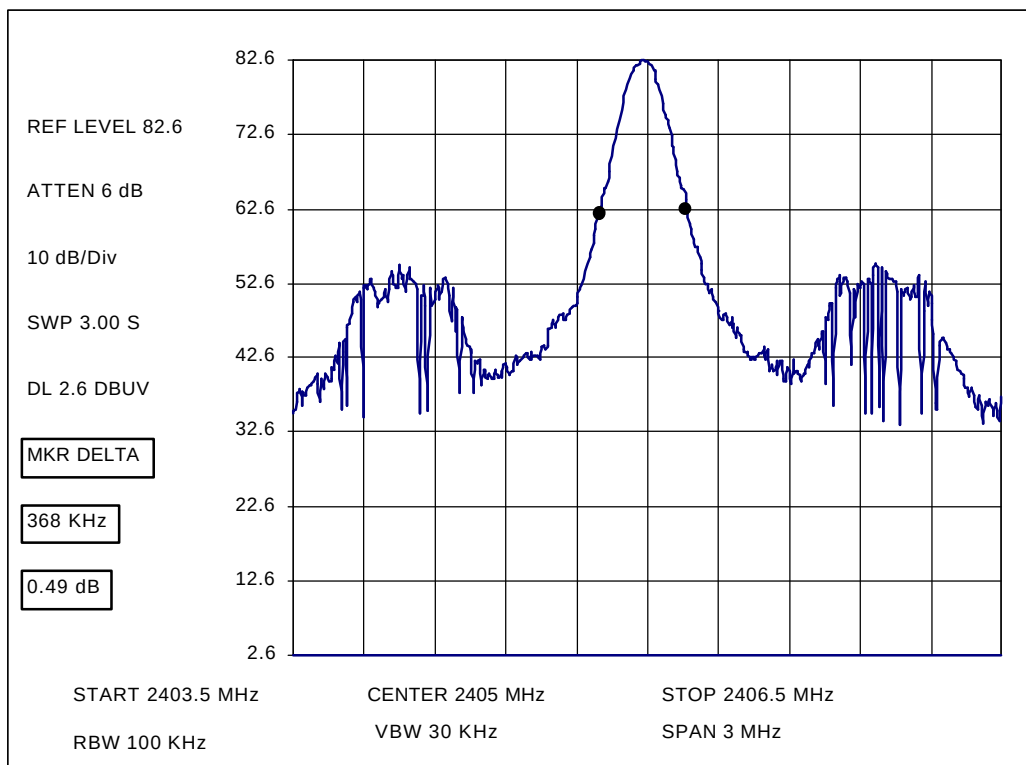
Plot 1: Low Channel 20 dB RF Bandwidth
