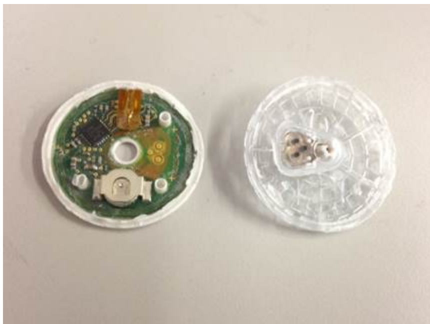
Photo 7 – Internal View of the Sensor
