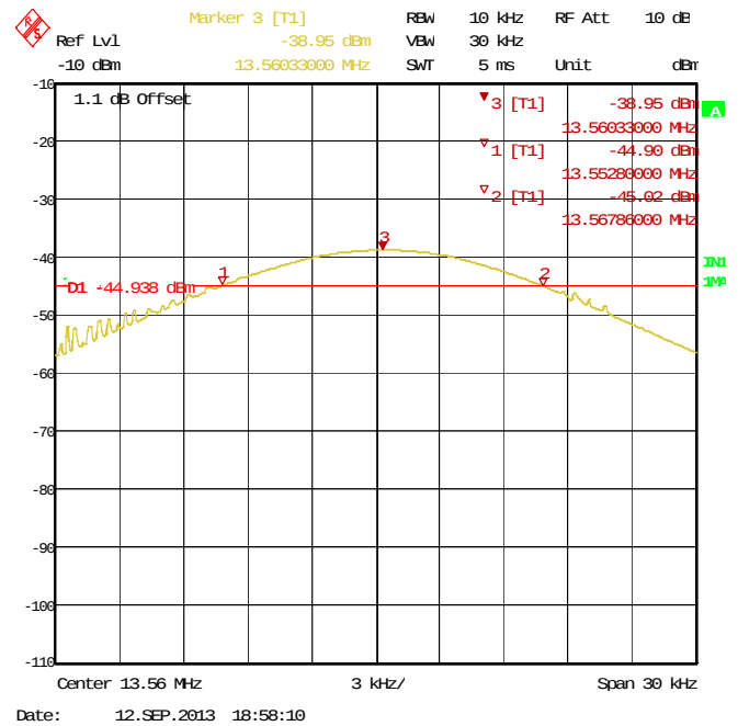
Figure 14: Frequency Stability at 20 °C - 2 min
