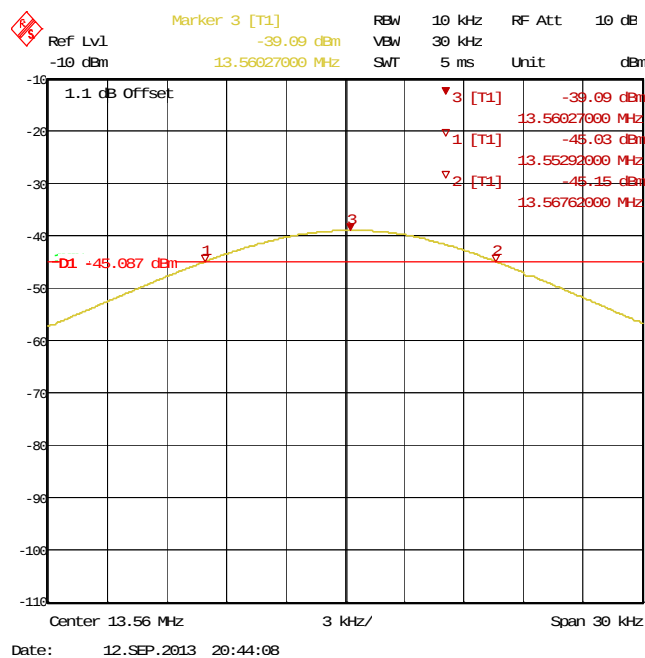
Figure 19: Frequency Stability at 30 °C - 5 min
