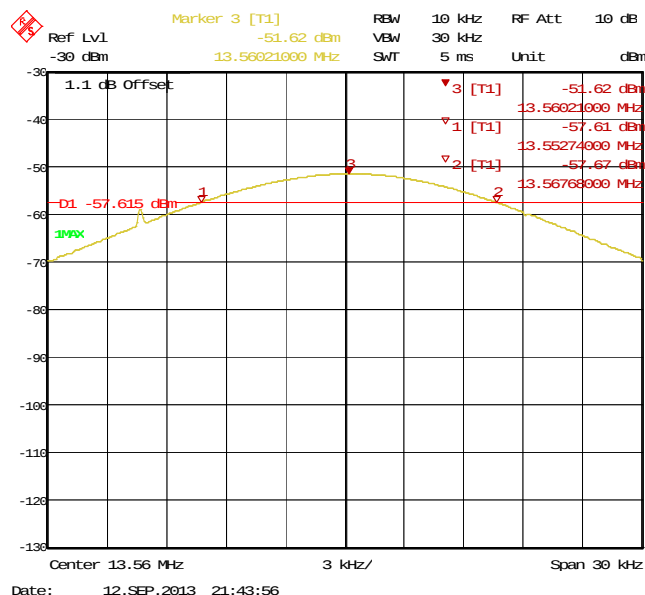
Figure 25: Frequency Stability at 45 °C - Start
