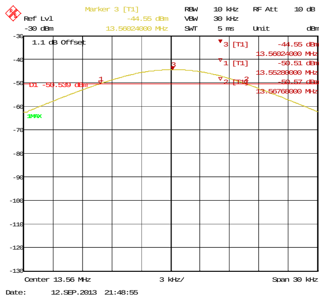
Figure 27: Frequency Stability at 45 °C - 5 min
