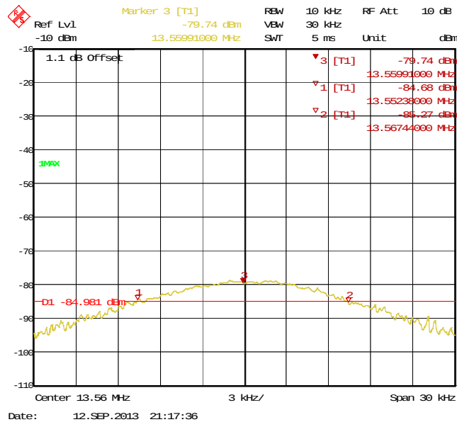
Figure 21: Frequency Stability at 40 °C - Start
