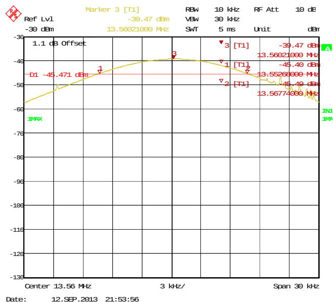
Figure 28: Frequency Stability at 45 °C - 10 min
