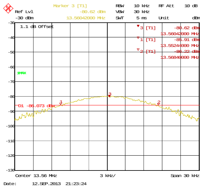
Figure 23: Frequency Stability at 40 °C - 5 min
