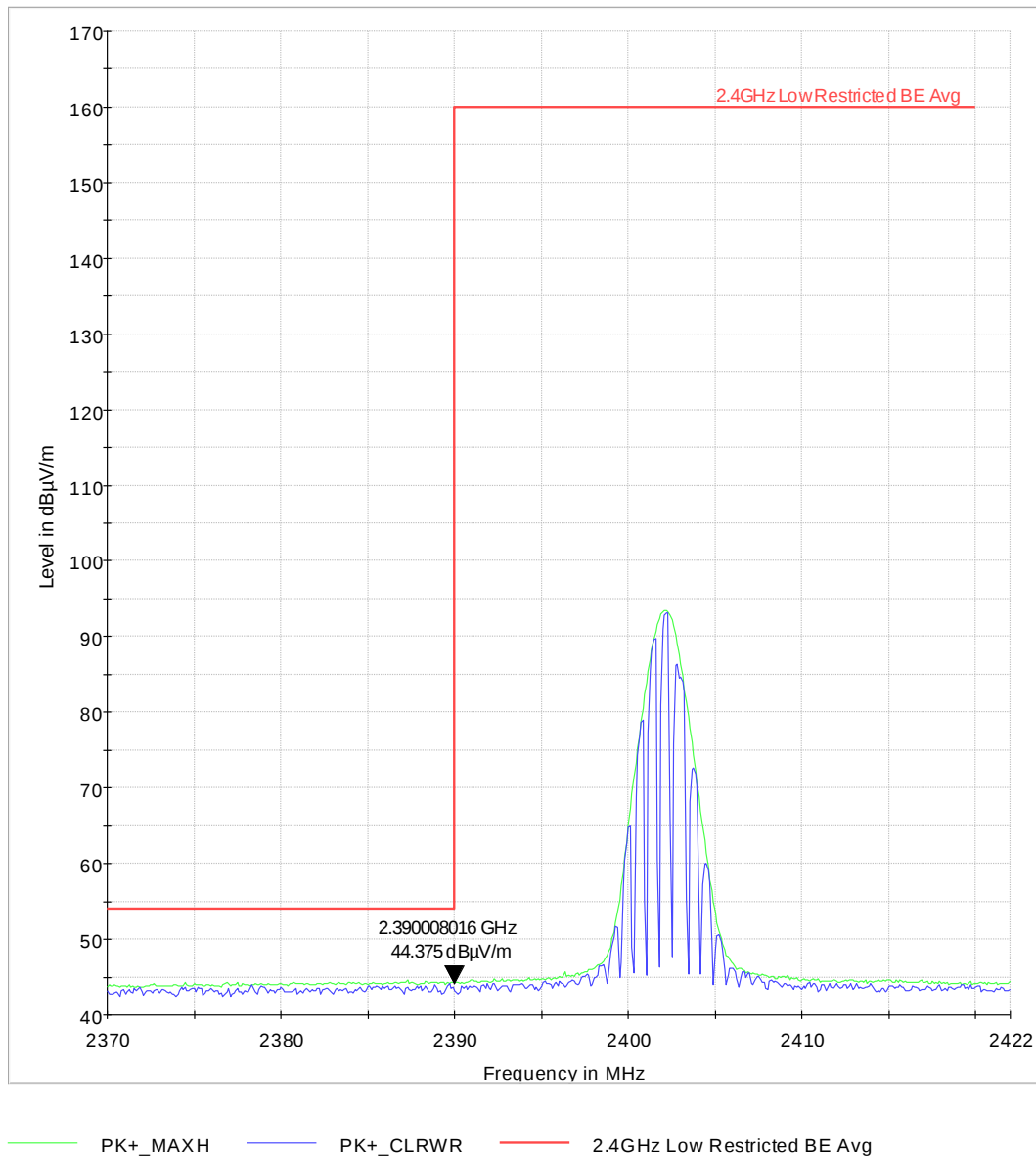
Figure 13: Low Channel Restricted Band Edge Average Detector– BT LE
