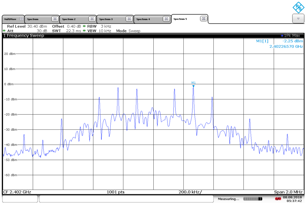
Figure 7: Power Spectral Density – BLE – 2402 MHz
