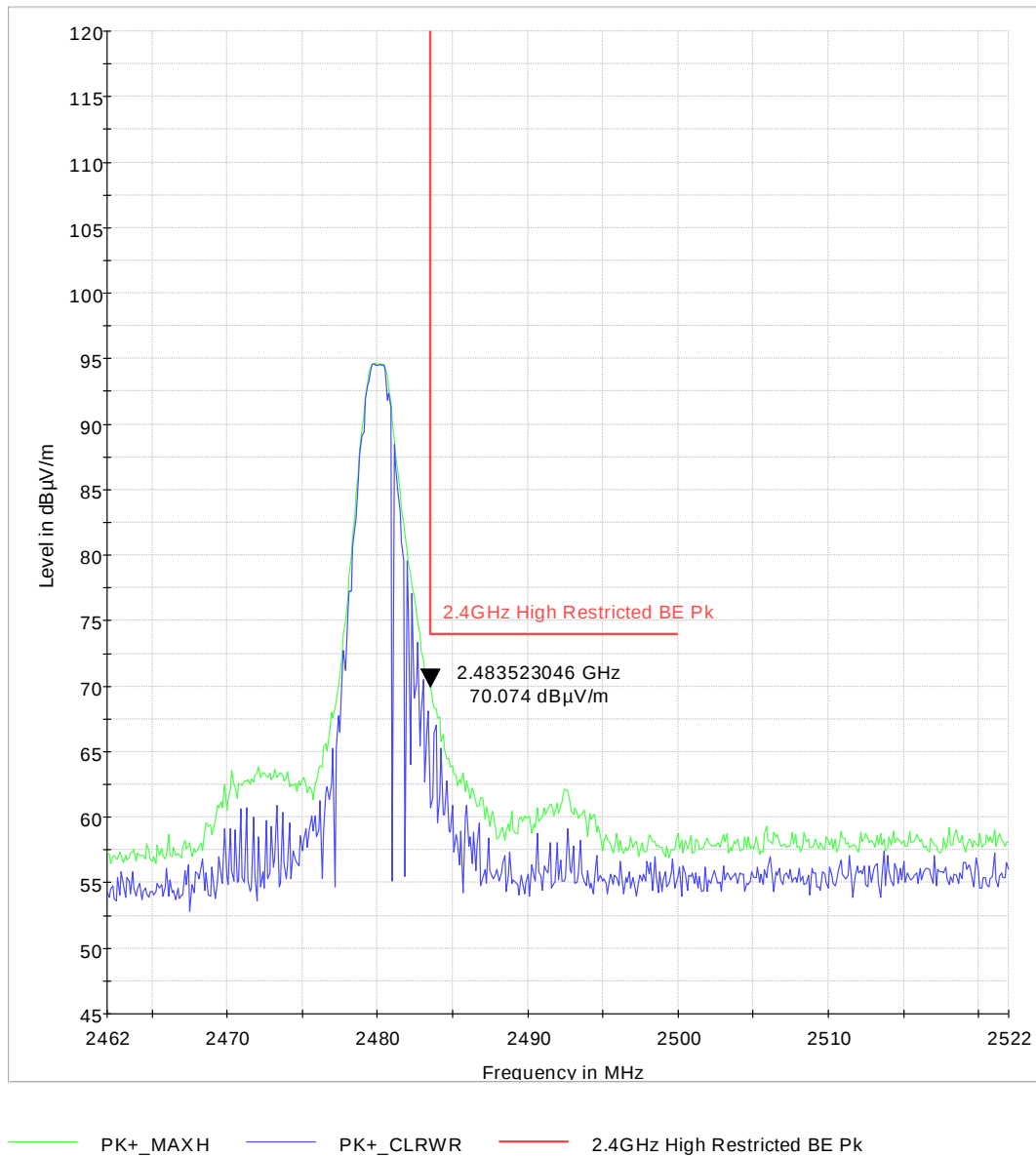
Figure 14: High Channel Restricted Band Edge Peak Detector– BT LE
