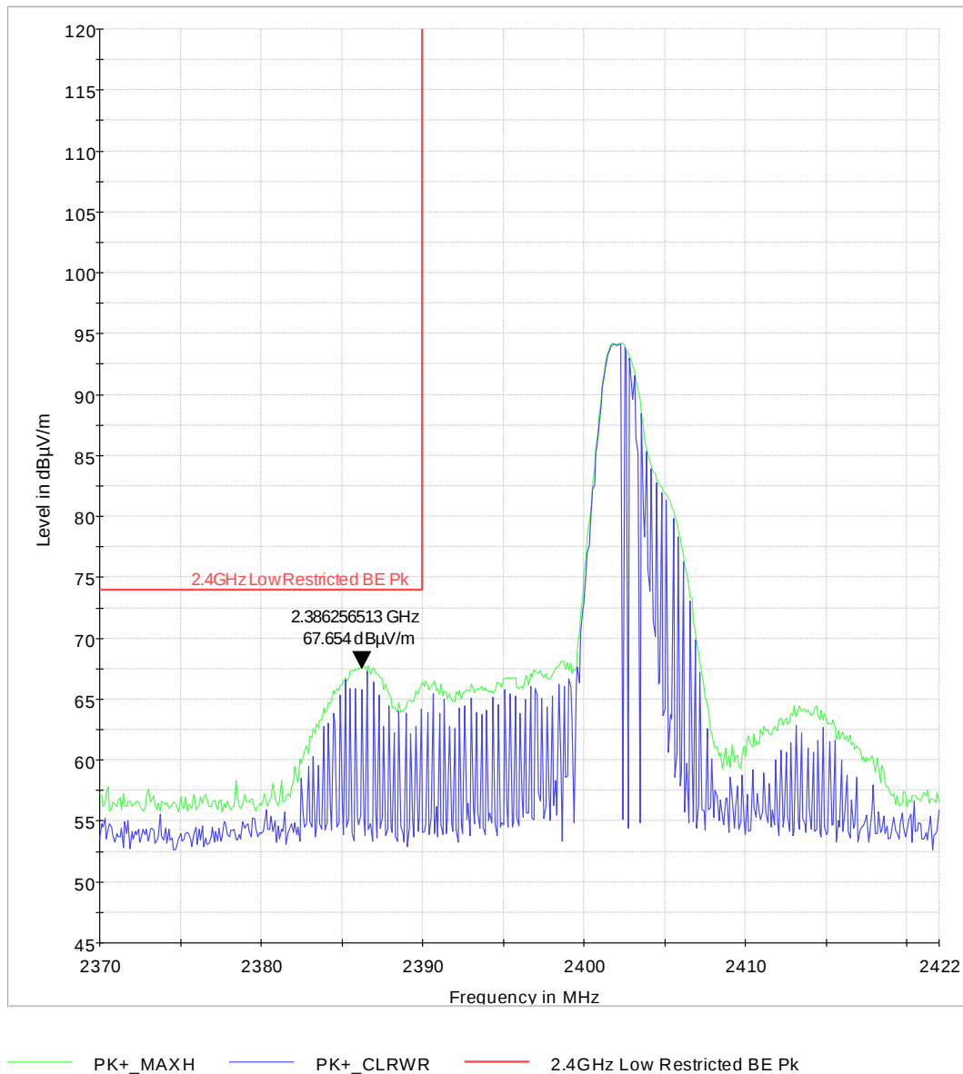
Figure 12: Low Channel Restricted Band Edge Peak Detector– BT LE
