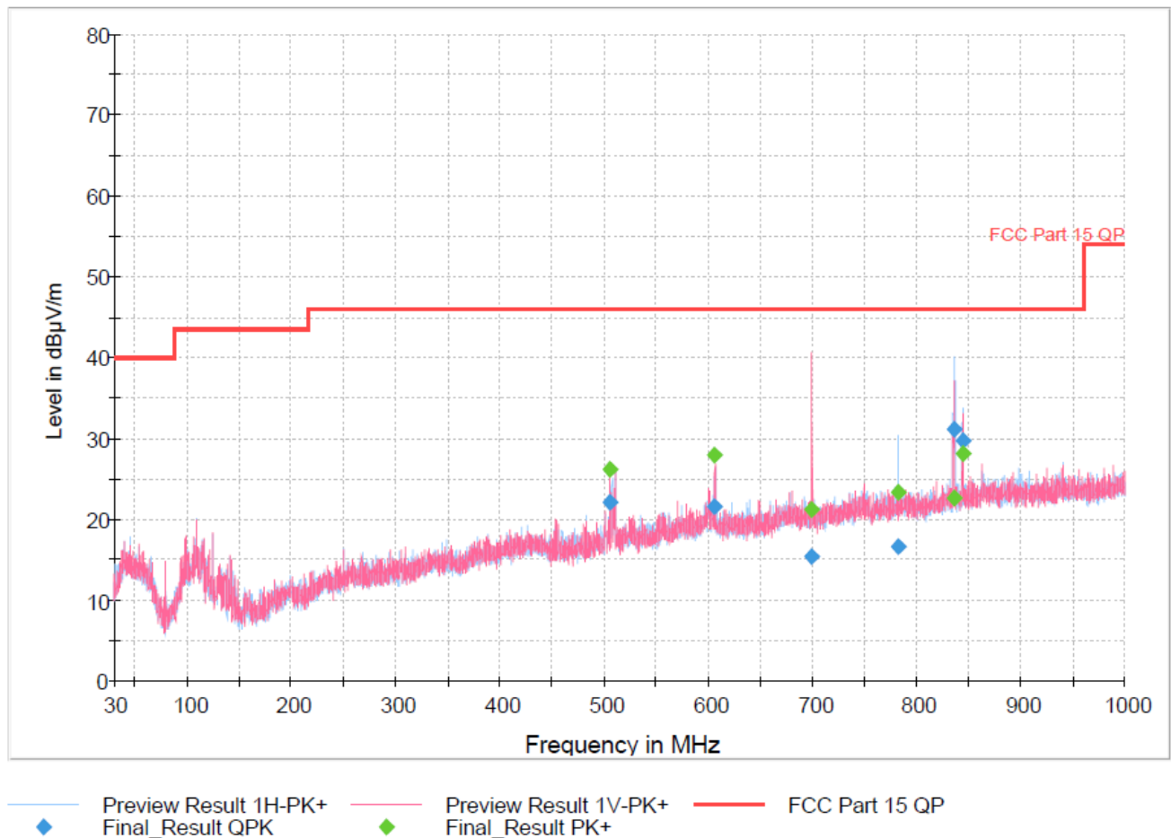
Plot 23. 30MHz-1GHz, BLE-2480MHz
