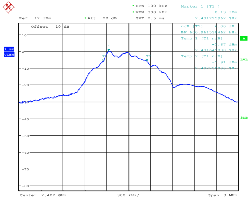
Plot 4. BLE-2402MHz, 6dB Bandwidth
