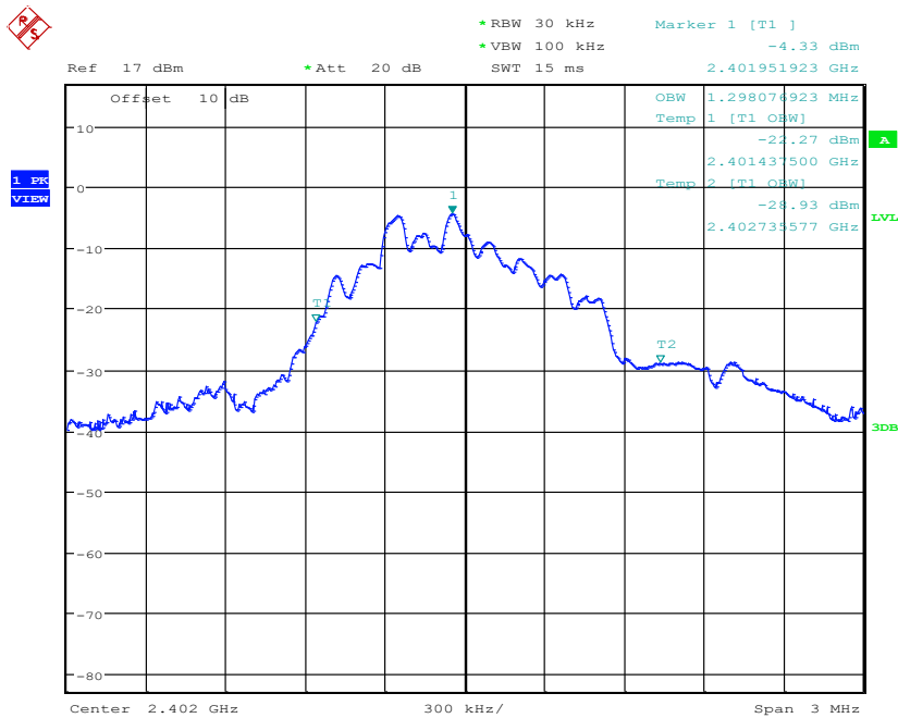
Plot 7. BLE-2402MHz, 99% Bandwidth
