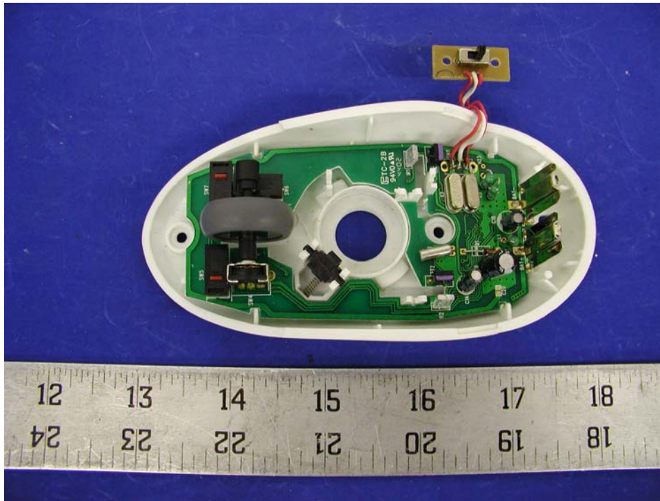
EUT – Cover Off View (PWB Side View 1)
