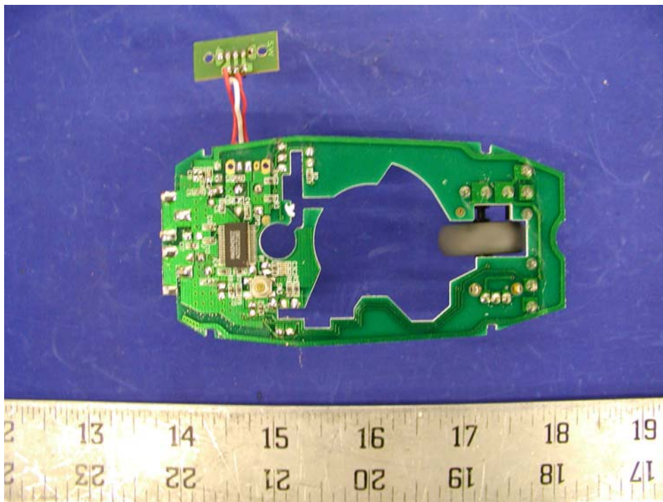
EUT – Main Board (PCB Side View 2)
