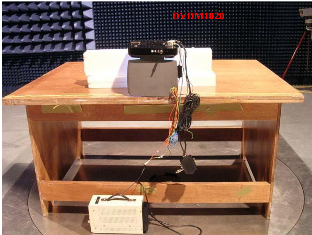
Photo 2: Radiated Emission Test Set-up photo
