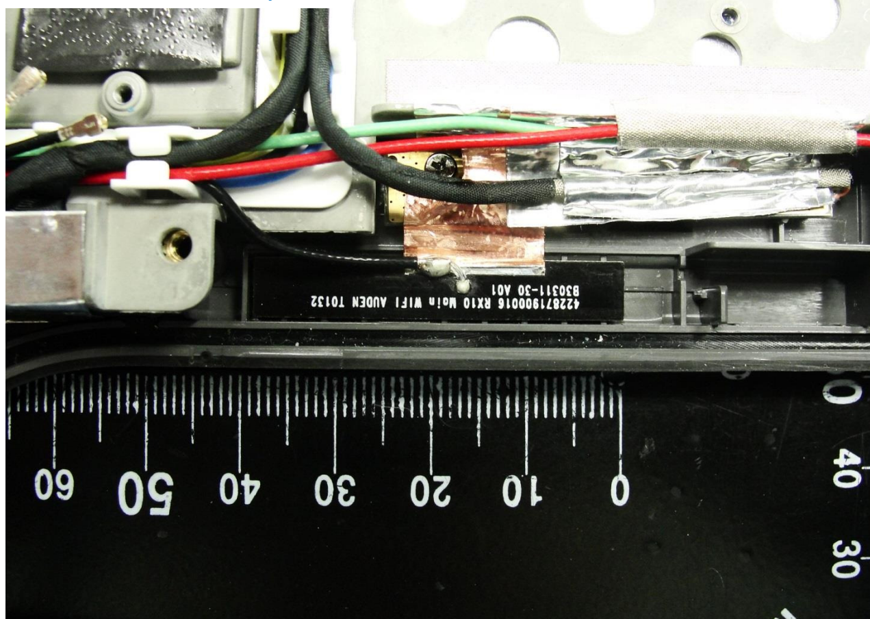
WLAN Main Antenna for Sample 3
