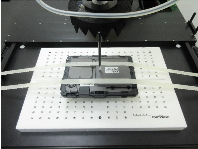
Testing Setup for Power Density, Bottom Surface at 0 mm Sample 1
