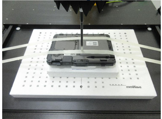
Testing Setup for Power Density, Bottom Surface of Antenna Side-1 at 0 mm Sample 1
