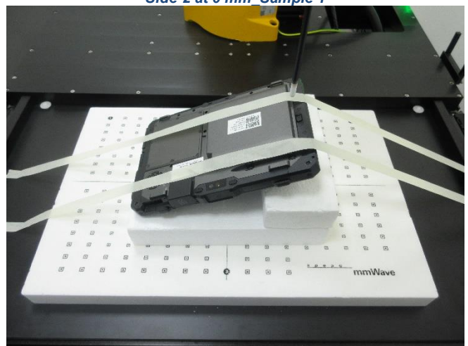
Testing Setup for Power Density, Bottom Surface of Antenna Side-2 at 0 mm Sample 1
