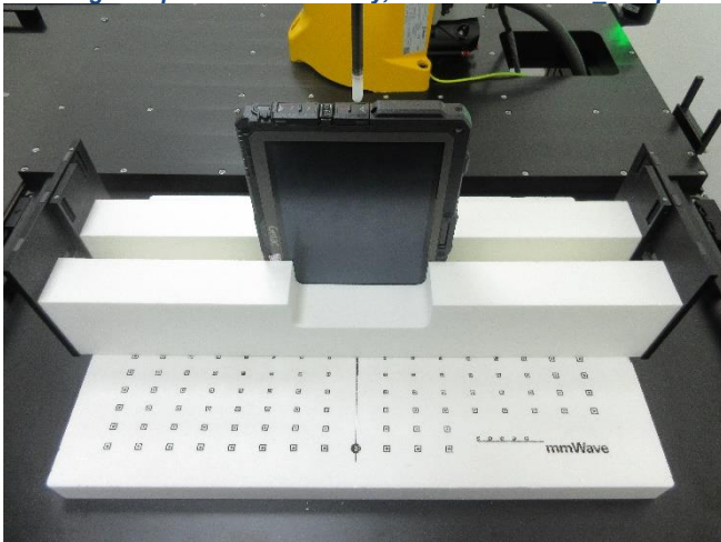
Testing Setup for Power Density, Left Side at 0 mm Sample 1
