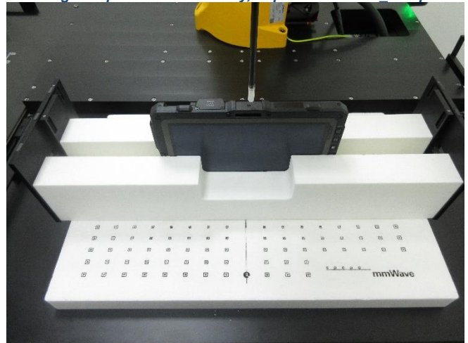
Testing Setup for Power Density, Top Side at 0 mm Sample 1
