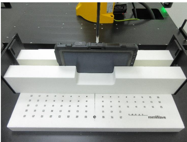
Testing Setup for Power Density, Top Side at 0 mm_Sample 2
