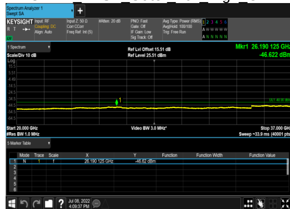
B13_N48(10M)_DFT-s-OFDM_QPSK Outer Full High CH
