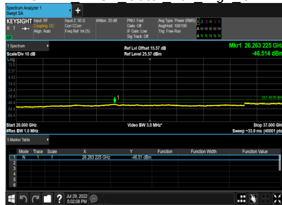
B13_N48(40M)_DFT-s- OFDM_QPSK_Outer_Full_High_CH
