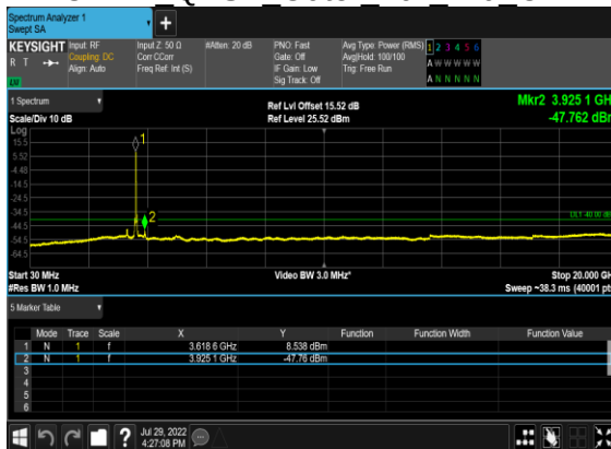
B13_N48(20M)_DFT-s-OFDM QPSK Outer Full Mid CH
