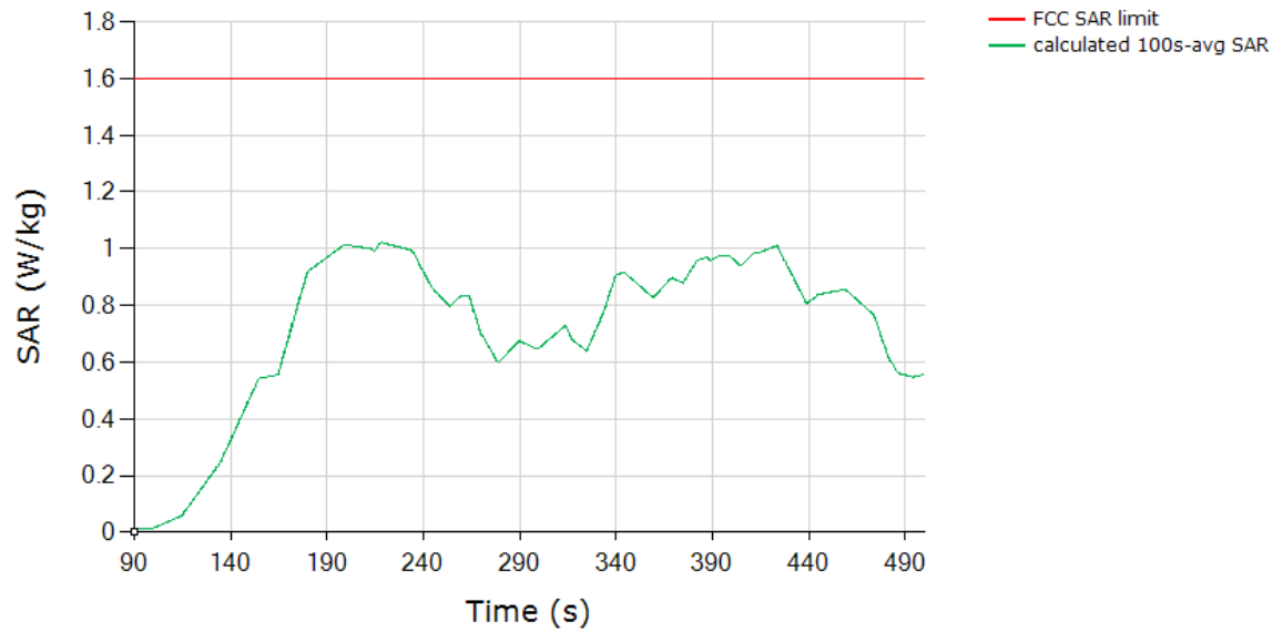
SAR (Test Sequence 2) Tech: LTE, Band 66
