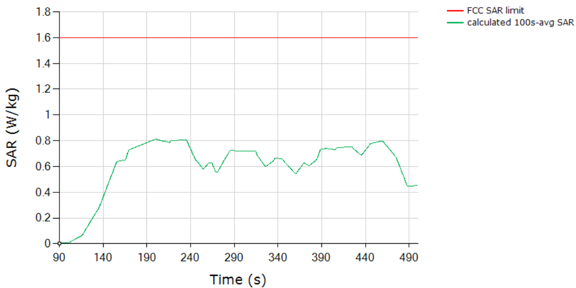
SAR (Test Sequence 2) Tech: 5GNR, Band 2
