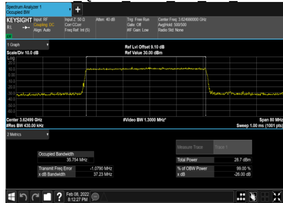
B13_N48(40M)_CP-OFDM_16 QAM Outer Full Mid CH
