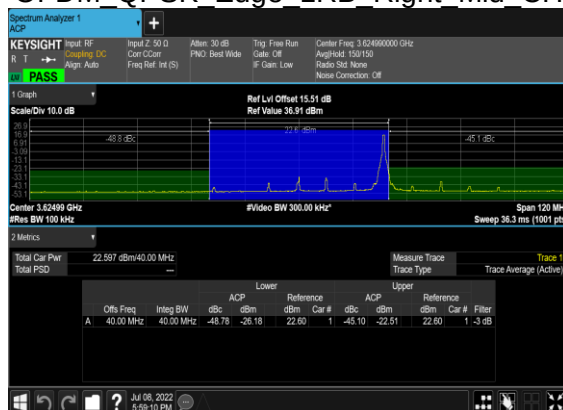
B13_N48(40M)_DFT-s-OFDM QPSK Edge 1RB Right Mid CH
