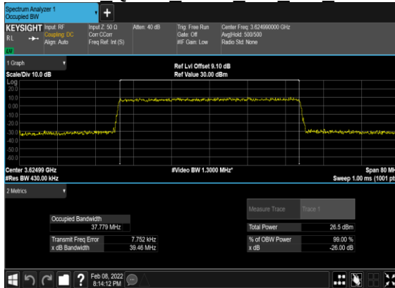
B13_N48(40M)_CP-OFDM_64 QAM Outer Full Mid CH
