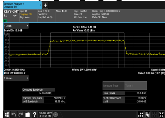
B13_N48(40M)_CP-OFDM_256 QAM Outer Full Mid CH
