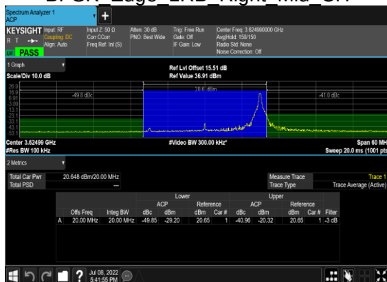
B13_N48(20M)_DFT-s-OFDM_PI_2-BPSK Edge 1RB Right Mid CH
