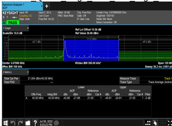
B13_N48(40M)_DFT-s-OFDM QPSK Edge 1RB Left High CH
