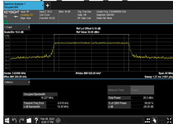
B13_N48(20M)_CP-OFDM_256 QAM Outer Full Mid CH
