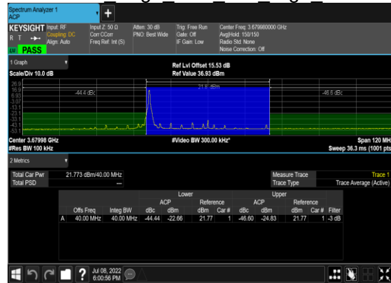
B13_N48(40M)_DFT-s-OFDM QPSK Outer Full High CH
