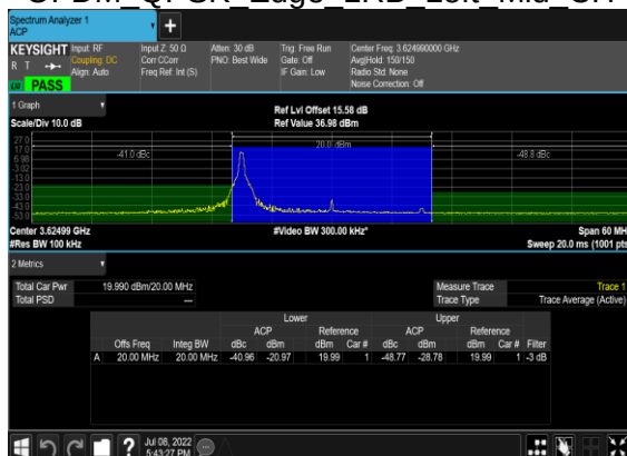
B13_N48(20M)_DFT-s-OFDM QPSK Edge 1RB Left Mid CH
