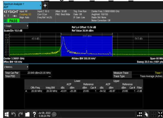
B13_N48(20M)_DFT-s-OFDM QPSK Outer Full Low CH
