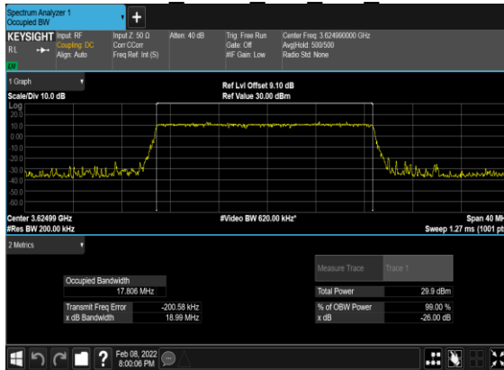
B13_N48(20M)_CP- OFDM QPSK Outer Full Mid CH
