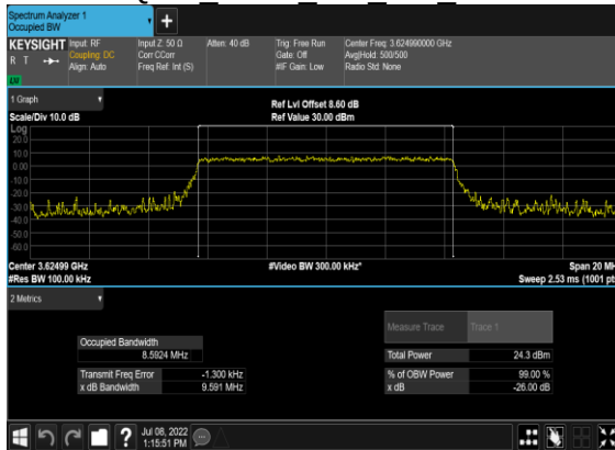
B13_N48(10M)_CP-OFDM_64 QAM Outer Full Mid CH
