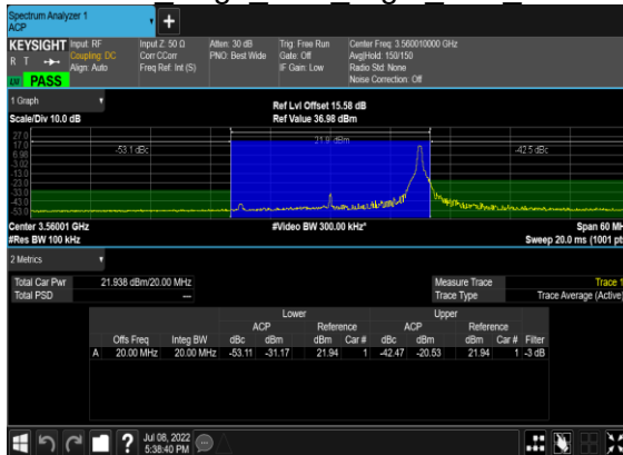
B13_N48(20M)_DFT-s-OFDM QPSK Edge 1RB Left Low CH
