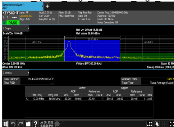
B13_N48(10M)_DFT-s-OFDM QPSK Edge 1RB Left High CH
