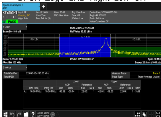
B13_N48(10M)_DFT-s-OFDM_PI_2-BPSK Edge 1RB Right Low CH
