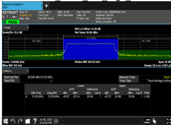
B13_N48(10M)_DFT-s-OFDM_PI_2-BPSK Edge 1RB Right High CH
