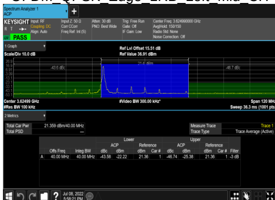
B13_N48(40M)_DFT-s-OFDM QPSK Edge 1RB Left Mid CH
