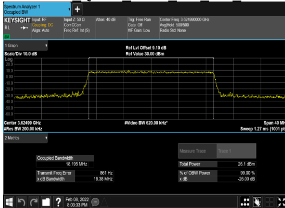
B13_N48(20M)_CP-OFDM_64 QAM Outer Full Mid CH
