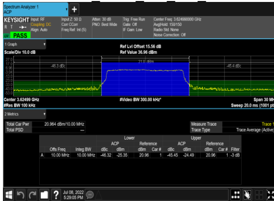
B13_N48(10M)_DFT-s-OFDM_PI_2-BPSK Edge 1RB Right Mid CH
