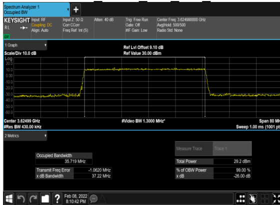
B13_N48(40M)_CP- OFDM QPSK Outer Full Mid CH
