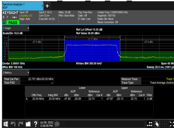
B13_N48(20M)_DFT-s-OFDM_PI_2-BPSK Edge 1RB Right Low CH
