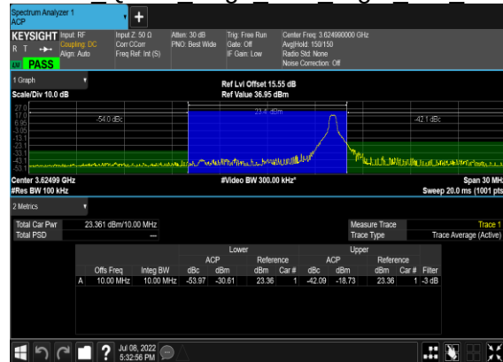
B13_N48(10M)_DFT-s-OFDM QPSK Edge 1RB Right Mid CH
