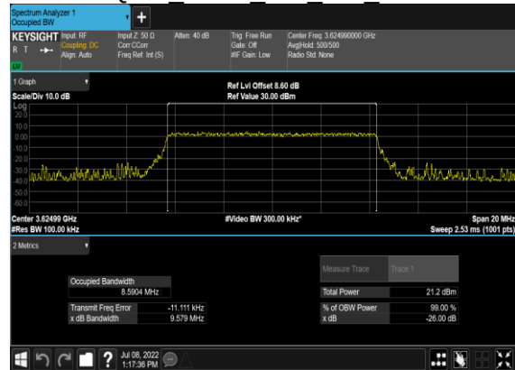
B13_N48(10M)_CP-OFDM_256 QAM Outer Full Mid CH
