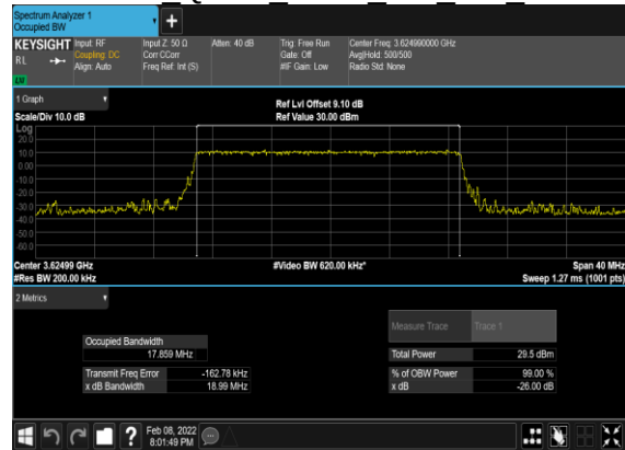
B13_N48(20M)_CP-OFDM_16 QAM Outer Full Mid CH
