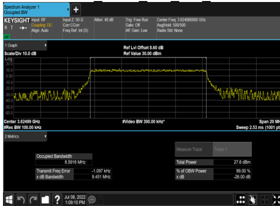
B13_N48(10M)_CP- OFDM QPSK Outer Full Mid CH
