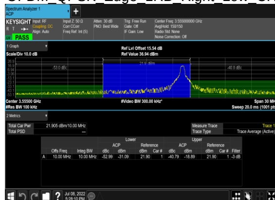
B13_N48(10M)_DFT-s-OFDM QPSK Edge 1RB Right Low CH
