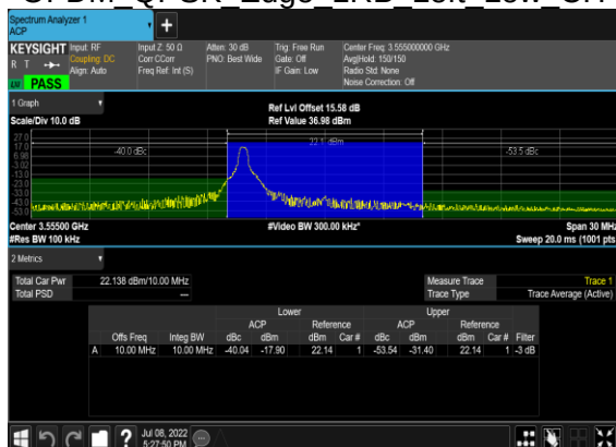
B13_N48(10M)_DFT-s-OFDM QPSK Edge 1RB Left Low CH
