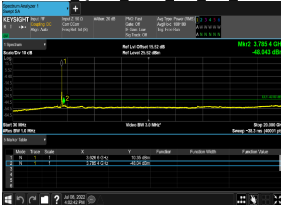
B13_N48(10M)_DFT-s-OFDM QPSK Outer Full Mid CH
