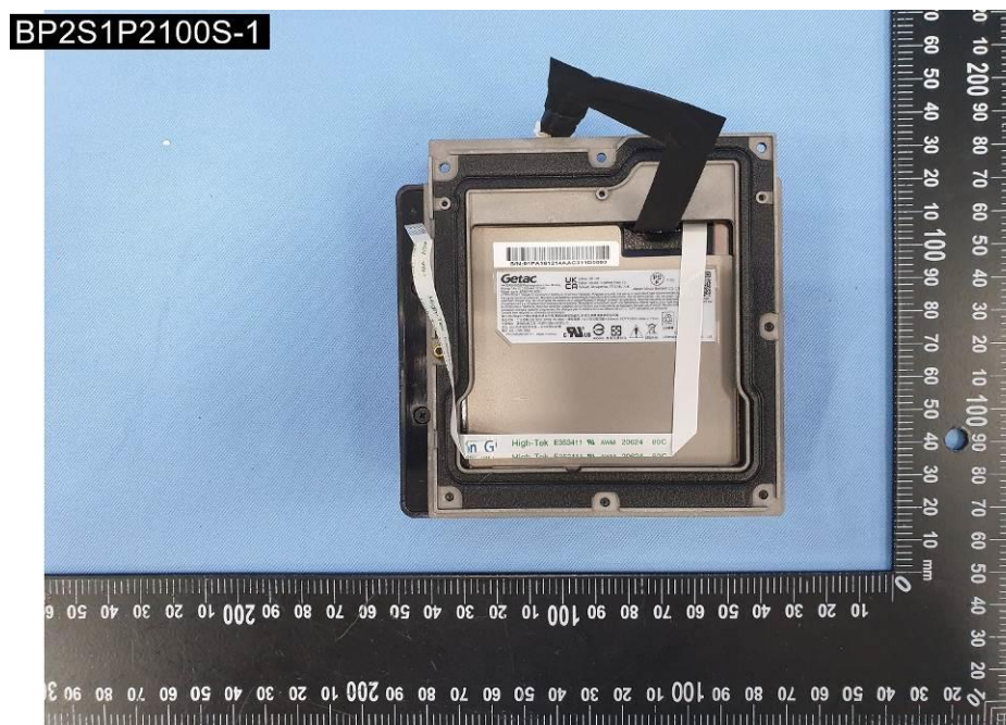
EUT Photo (32)
