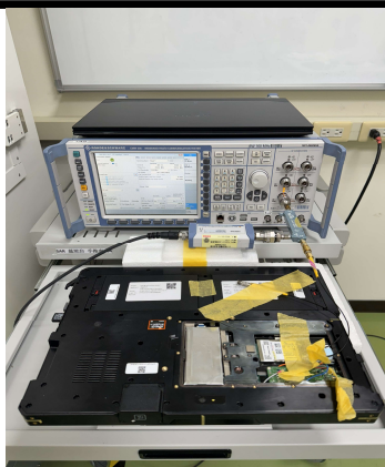
Setup for Conducted Power Test (for WCDMA / LTE Band)
