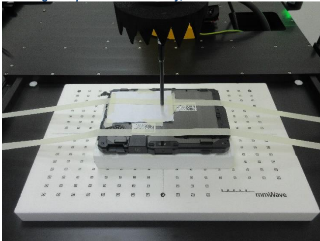
Testing Setup for Power Density, Bottom Surface at 2 mm
