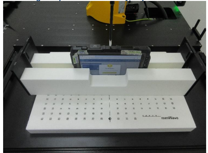
Testing Setup for Power Density, Top Side at 2 mm
