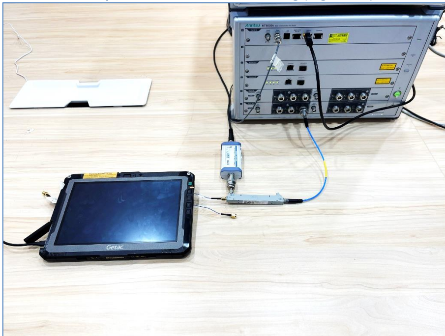
Setup for Conducted Power Testing (Figure 4-4)
