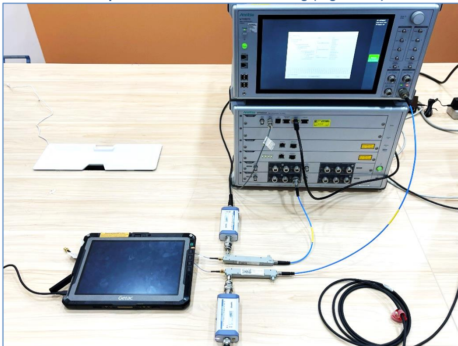
Setup for Conducted Power Testing (Figure 4-6)
