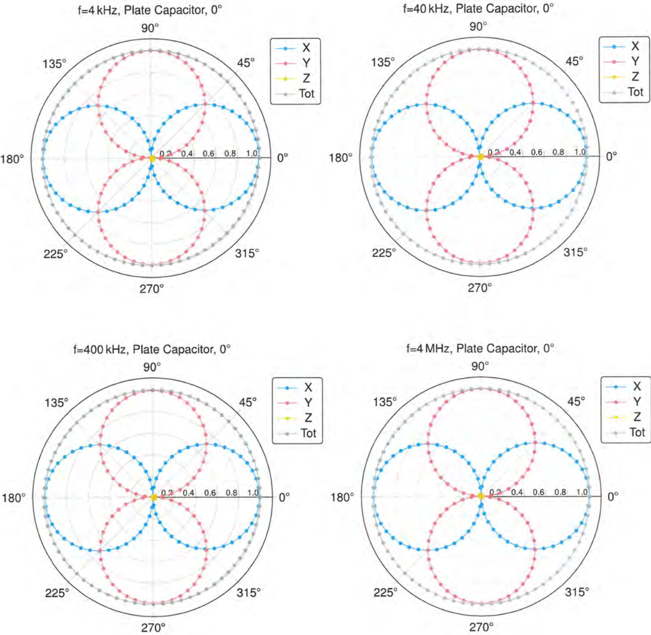
E-Field Receiving Pattern ( \phi ), \vartheta = 0^\circ
