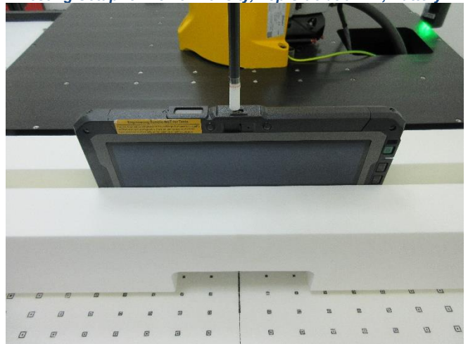
Testing Setup for Power Density, Top Side at 0 mm, Battery2
