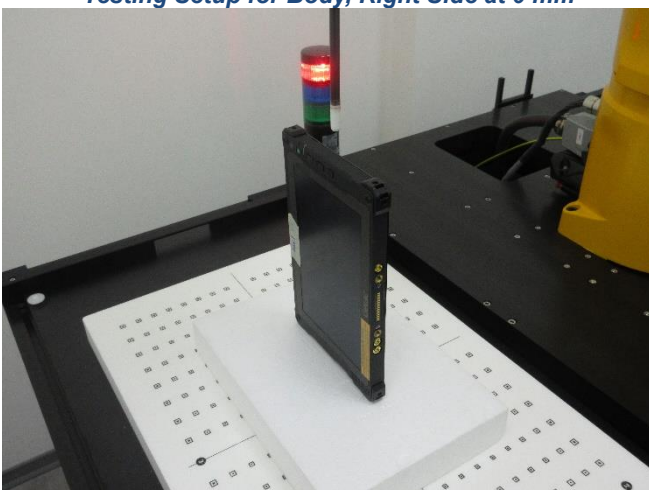
Testing Setup for Body, Right Side at 0 mm
