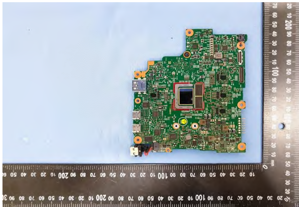
EUT Photo (39)
