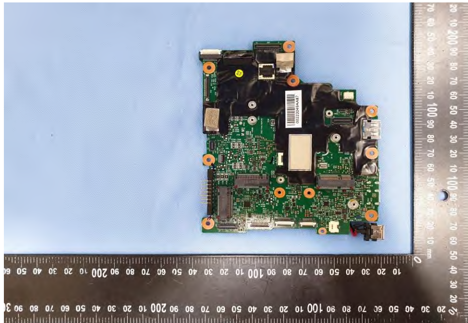
EUT Photo (43)
