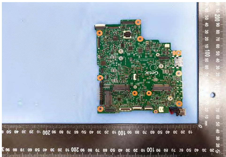
EUT Photo (43)
