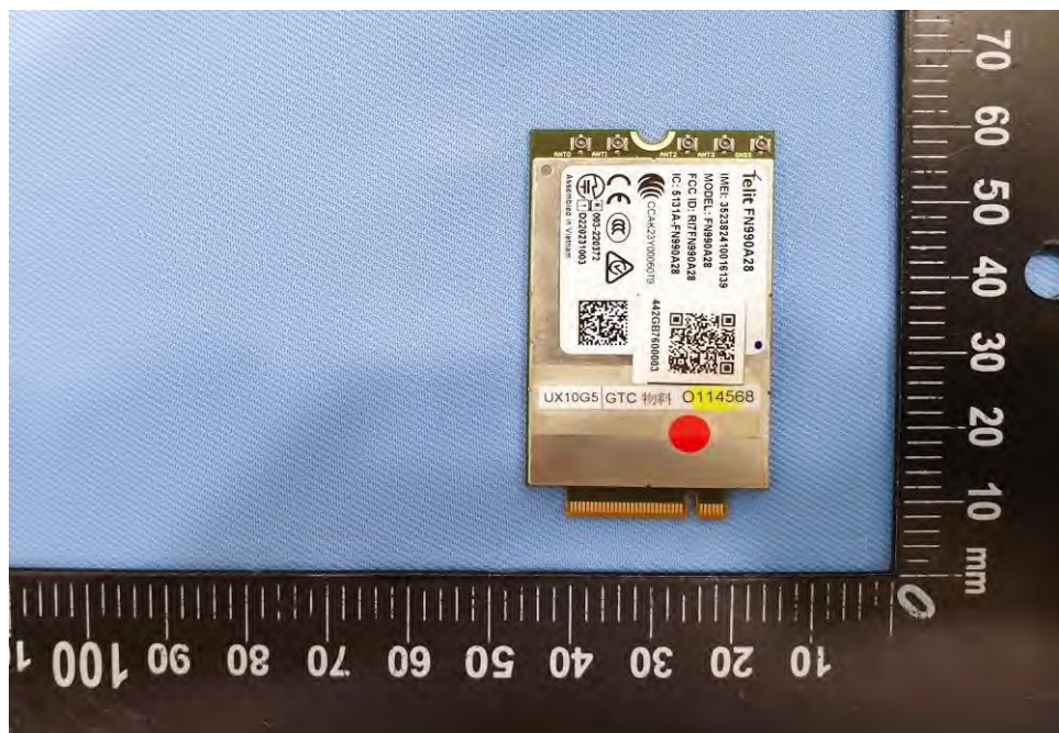
EUT Photo (25)
