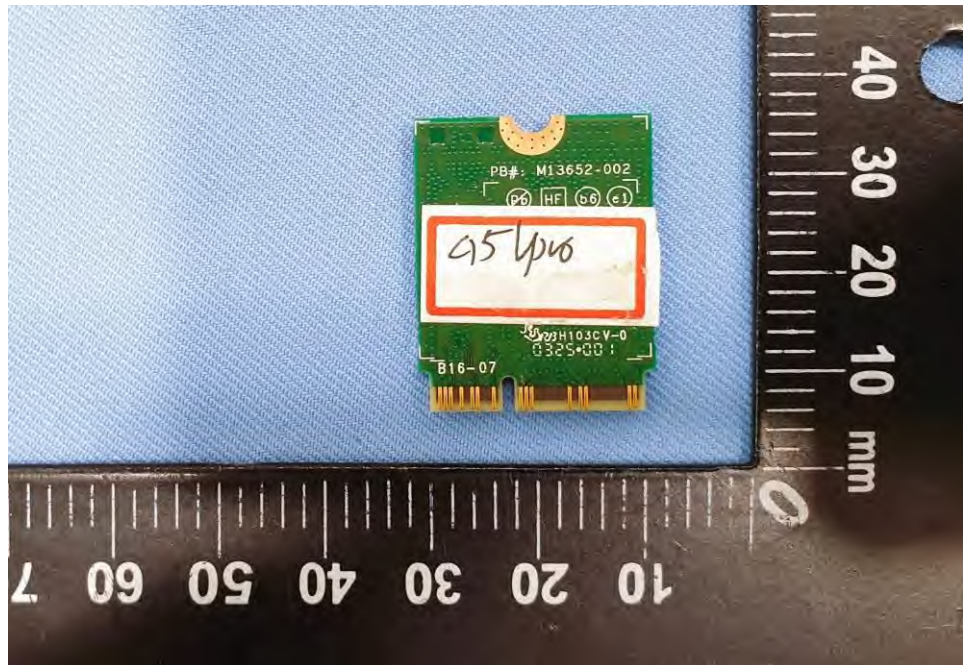
EUT Photo (25)
