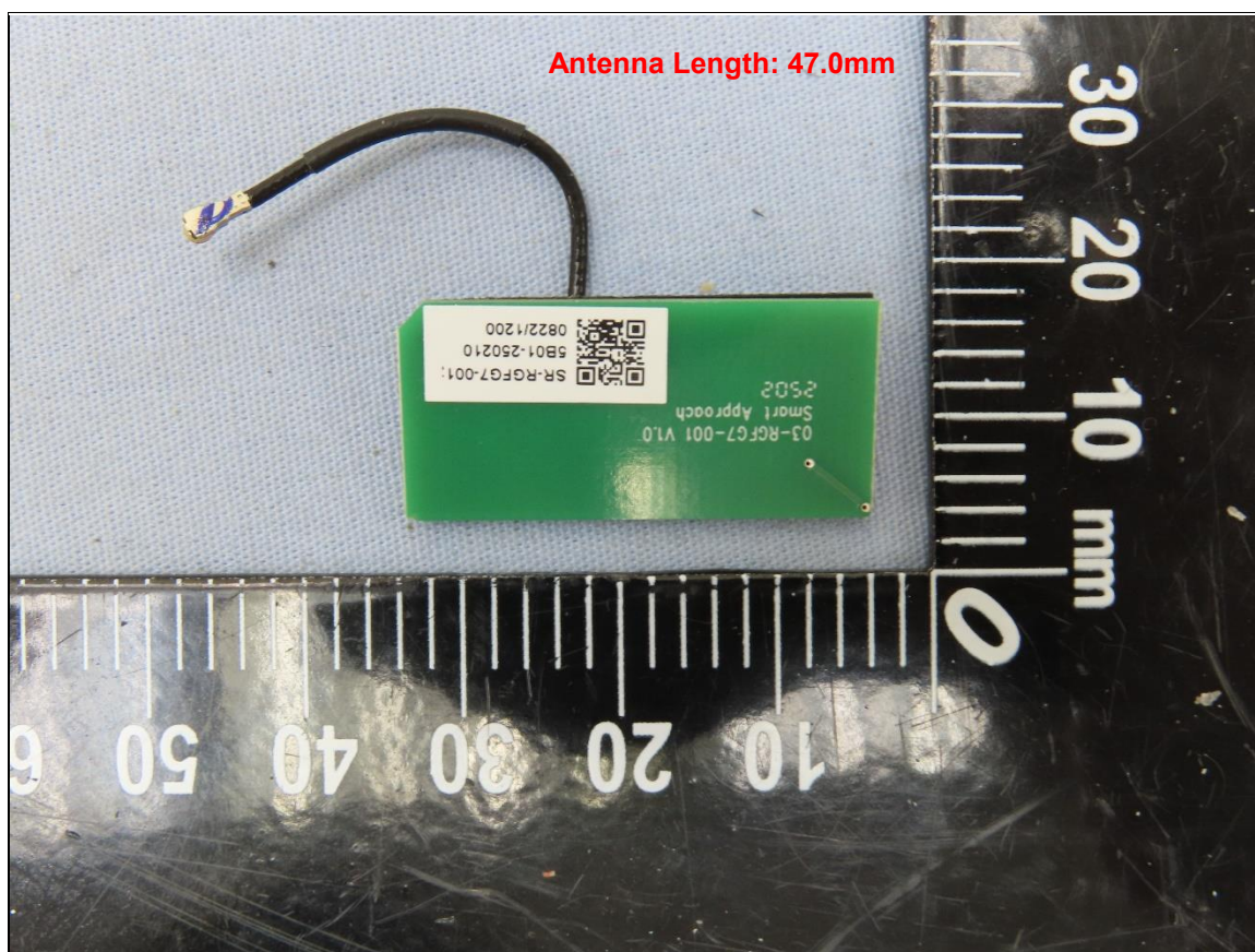
RFID Antenna, Brand: Smart Approach, Model: SR-RGFG7-001
